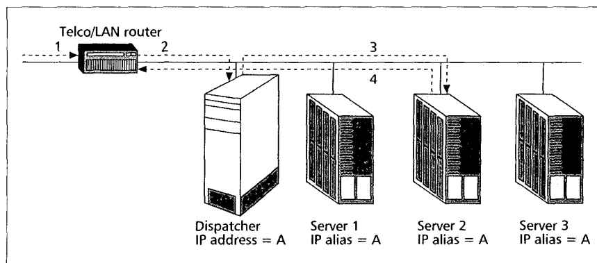
■ Figure 3. Traffic flow in an L4/2 cluster.
