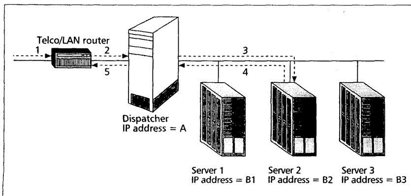
■ Figure 5. Traffic flow in an L4/3 cluster.
