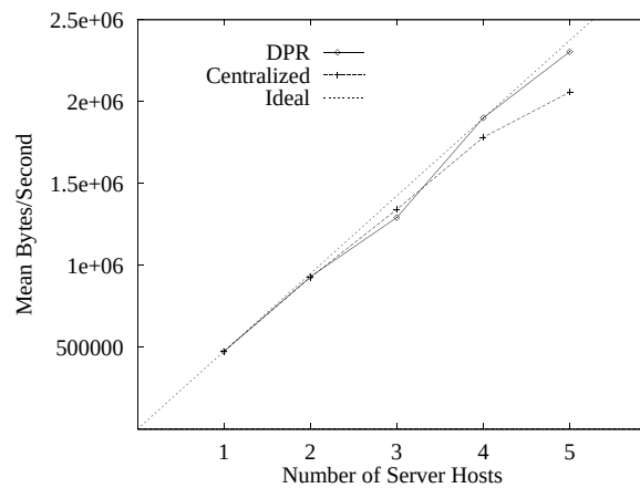
Figure 5. Scalability Comparison
