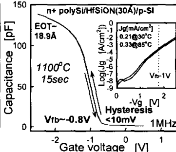
Fig.14. C-V and J-V characteristics of n+poly-Si/HfSiON/p-Si structure.
