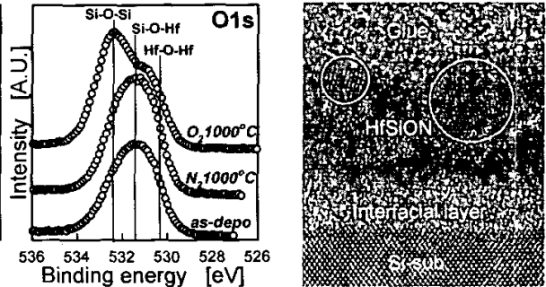
Fig.11. Chemical stability of Hf-O-Si bonds in HfSiON.
