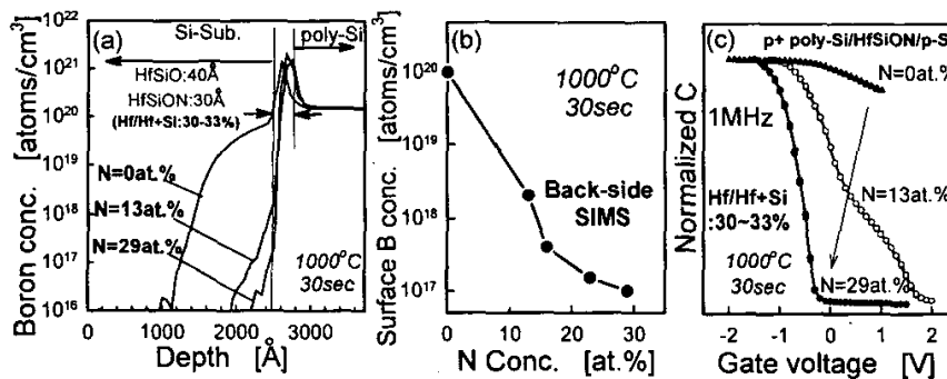
Fig.16. Suppression of B penetration into Si substrate through HfSiON measured by back-side SIMS((a)(b)). Improvement in C-V curve due to the suppression of B penetration is also demonstrated((c)).
