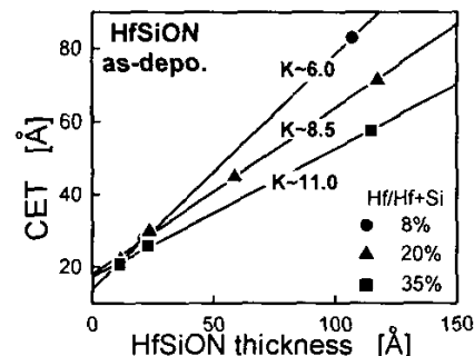
Fig. 3. Evaluation of dielectric constant of HfSiON films.
