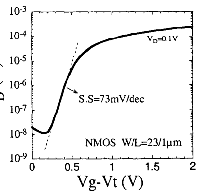
Fig. 13. I_d - V_g characteristics of NMOSFET ( \text{HfO}_2 gate stack with n^+ -poly Si gate).
