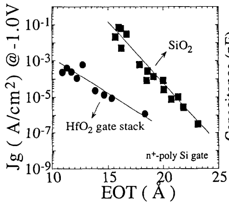
Fig. 3. Current density @ Vg=-1V as a function of EOT for HfO 2 and SiO 2 with n + -poly Si gate.
