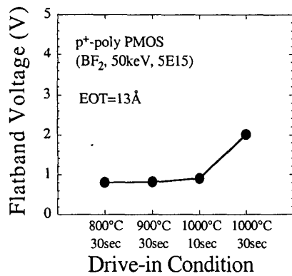
Fig. 11. Boron penetration characteristics of \text{HfO}_2 gate stack by flatband voltage shift during gate activation.
