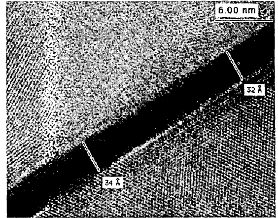
Fig. 8. TEM picture of \text{HfO}_2 gate stack with a-Si gate doped with P-implant (Gate Activation : 900^\circ\text{C} , 60sec + 950^\circ\text{C} , 60sec).
