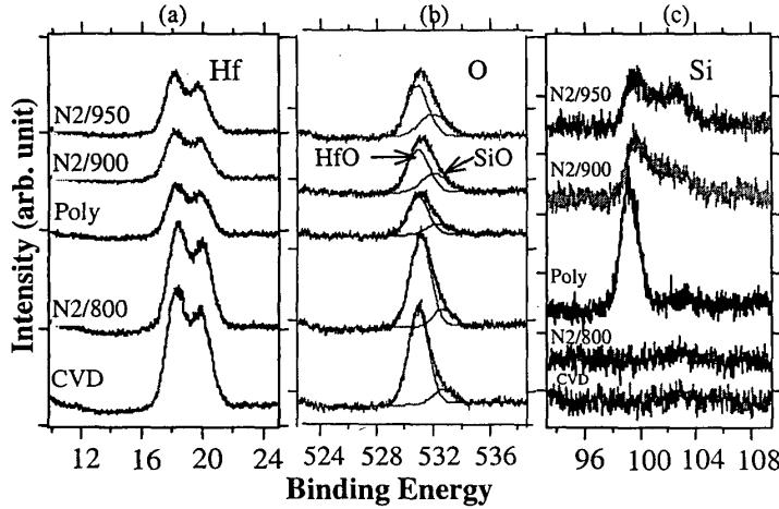
Fig. 7. XPS analysis of (a) Hf 4f, (b) O 1s and (c) Si 2p of \text{HfO}_2 gate stack deposited on clean Si(100) at 450^\circ\text{C} for 2min followed by \text{N}_2 annealing at 800^\circ\text{C} for 1min, poly-Si deposition at 600^\circ\text{C} and \text{N}_2 annealing at 900^\circ\text{C} and 950^\circ\text{C} for 30sec.
