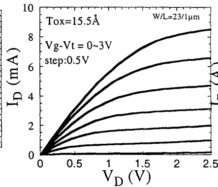
Fig. 12. I_d - V_d characteristics of NMOSFET ( \text{HfO}_2 gate stack with n^+ -poly Si gate).
