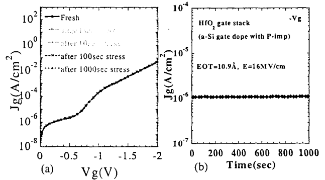
Fig. 10. (a) J_g - V_g after constant voltage stress (b) J_g -Time during constant voltage stress of \text{HfO}_2 gate stack with a-Si gate doped with Phosphorus implantation.
