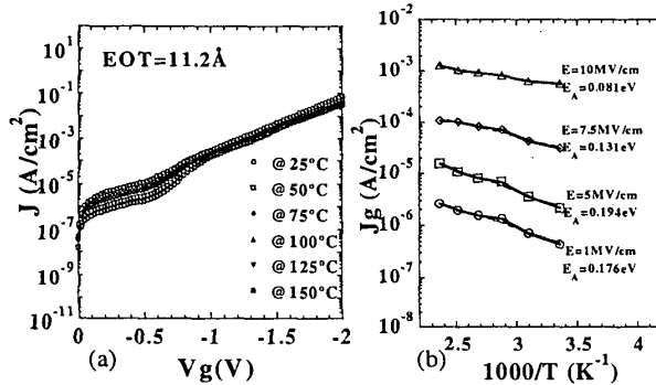
Fig. 9. (a) J_g - V_g at different temperature (b) Arrhenius's plot of temperature dependent leakage current of \text{HfO}_2 gate stack with a-Si gate doped with Phosphorus implantation.
