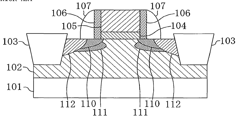
FIG. 16B PRIOR ART
