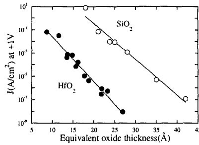
Fig. 11 At the same EOT, HfO 2 films show lower leakage current than conventional SiO 2 .
