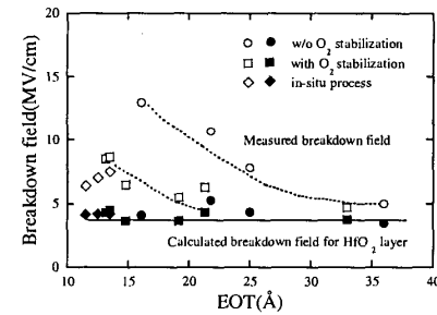
Fig. 17 Modeled breakdown field for HfO 2 layer showing that the actual breakdown field is around -4MV/cm.
