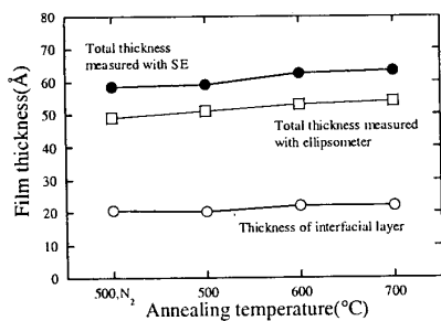
Fig. 6 Interfacial layer thickness measured with spectroscopic ellipsometer.
