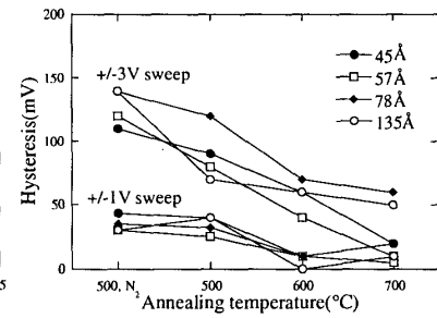
Fig. 12 Hysteresis of HfO 2 decreases as the annealing temperature increases.
