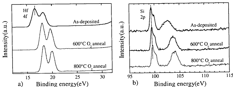
Fig. 9 Binding energy shift of 45 Å HfO 2 after annealing; a) Hafnium peak, b) Silicon peak.
