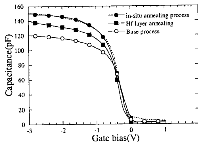
Fig. 4 Typical CV curve of HfO 2 capacitor showing the effect of oxygen supply control. Dashed line is a modified device accounting quantum mechanical effect.
