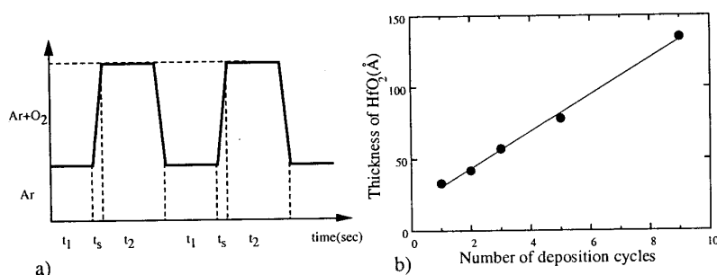
Fig. 1 Reactive dc magnetron sputtering process; a) Schematic diagram of process ( t_1 period = Ar ambient, t_2 = Ar+O 2 ambient, t_s = O 2 flow stabilization period), b) Film thickness is linearly proportional to the process cycles.
