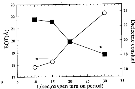
Fig. 2 The effect of oxidation time t_2 on EOT with a fixed t_1 . Dielectric constant of HfO 2 layer drops when oxidation time t_2 is excessive.
