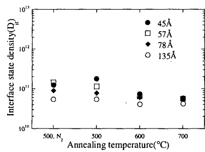
Fig. 14 Interface state density determined by Terman method.
