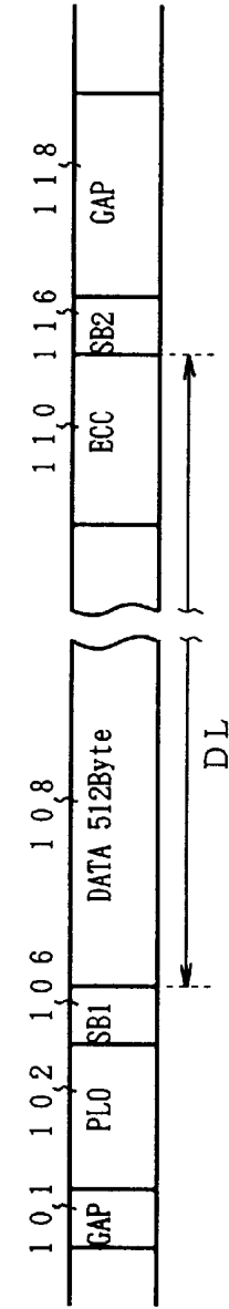
FIG. 8A MEDIUM DATA FORMAT
