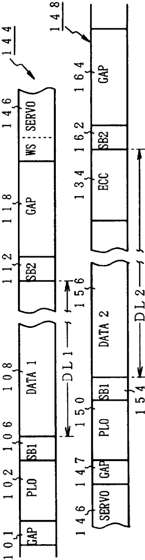
FIG. 11A MEDIUM DATA SPLIT-FORMAT
