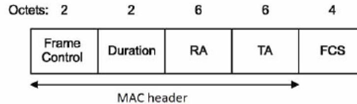
Figure 9-20—RTS frame
