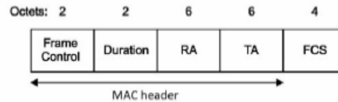
Figure 9-20—RTS frame
