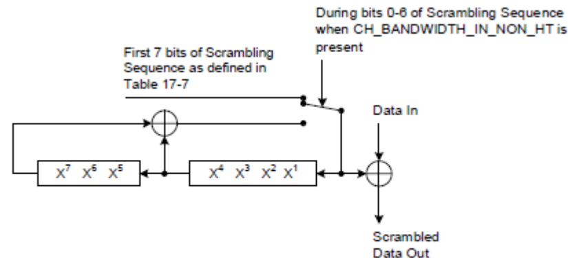
Figure 17-7—Data scrambler
