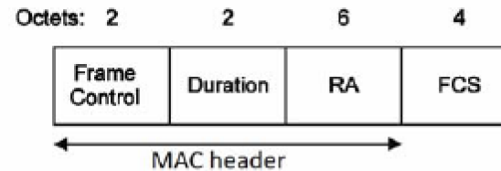
Figure 9-21—CTS frame
