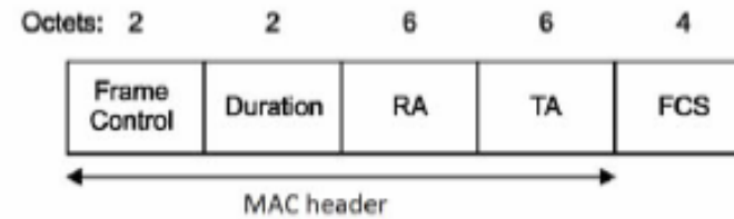
Figure 9-20—RTS frame
