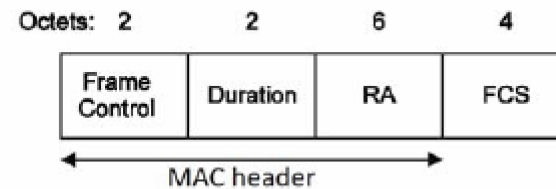
Figure 9-21—CTS frame
