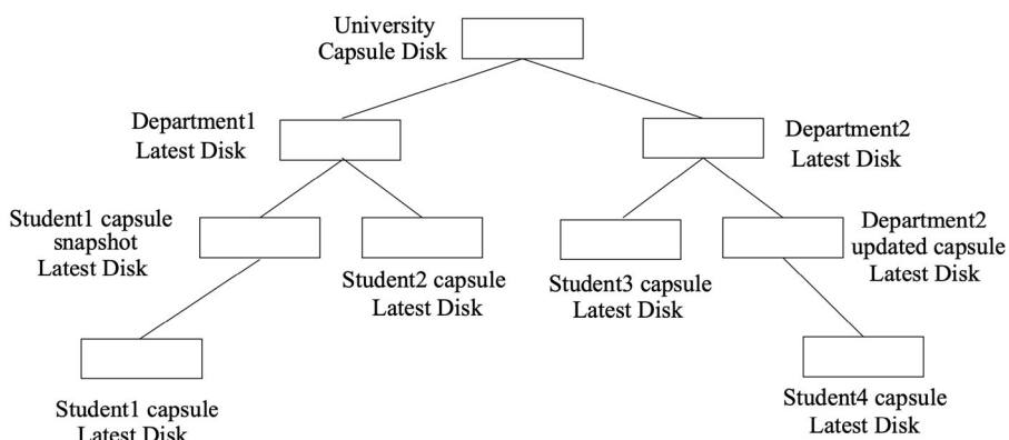
Figure 1: An example capsule hierarchy.
