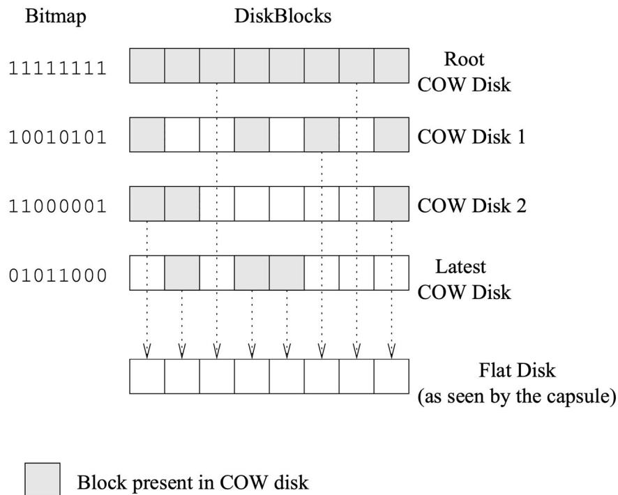
Figure 2: An example capsule disk.
