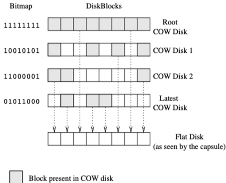
Figure 2: An example capsule disk.
