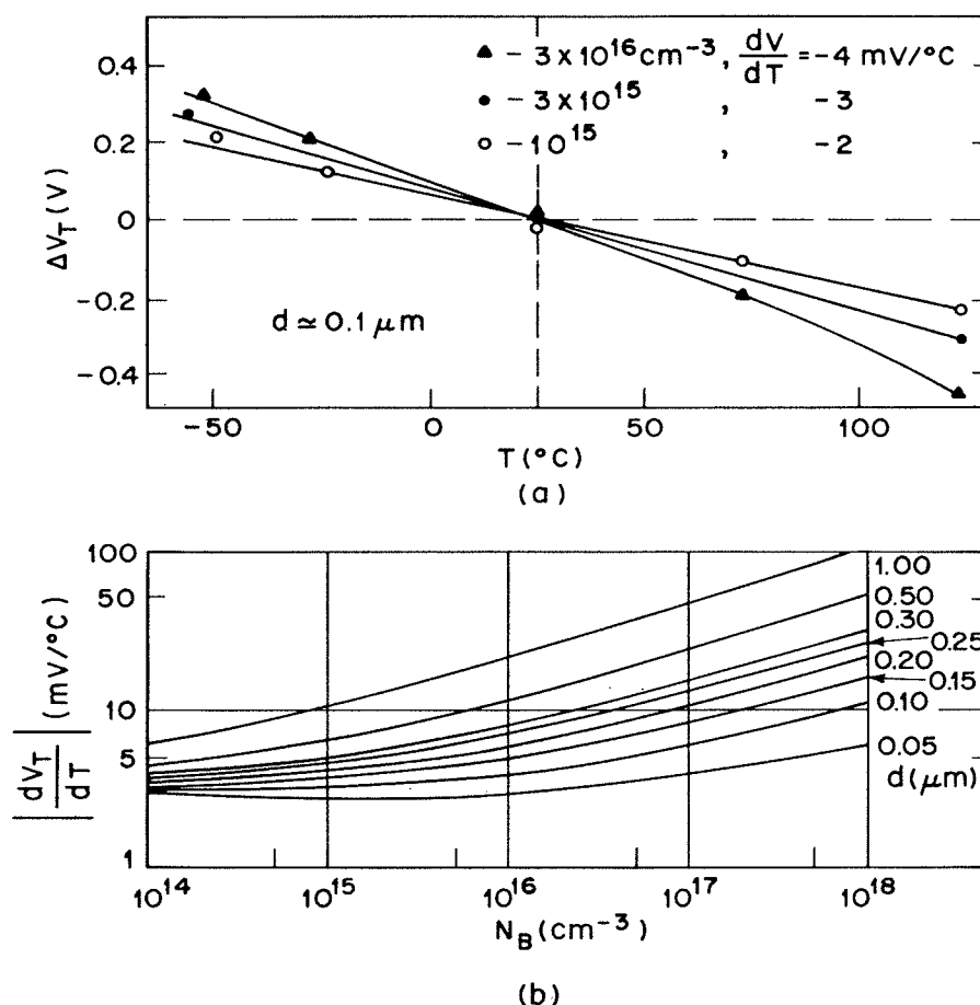
Fig. 16 (a) Experimental measurement of threshold voltage versus temperature. (b) dV_T/dT of a Si-SiO 2 system versus substrate doping with oxide thickness as a parameter. (After Vadasz and Grove, Ref. 29; Wang et al., Ref. 30.)
