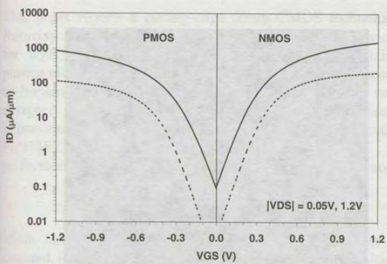
Figure 6: Sub-threshold curves for 35nm Lgate devices
