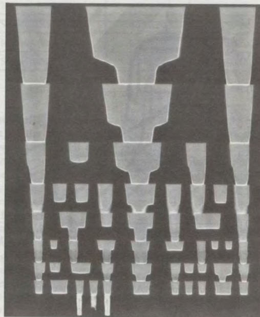
Figure 10: Cross-section: the dual damascene interconnects
