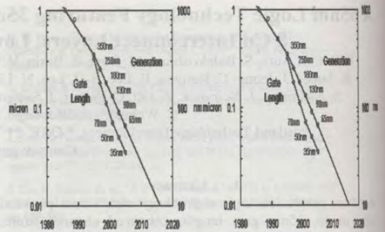
Figure 2: Transistor size trend for technology nodes.
