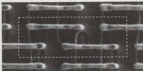
Figure 12: 0.57 \mu\text{m}^2 6-T SRAM cell at poly layer
