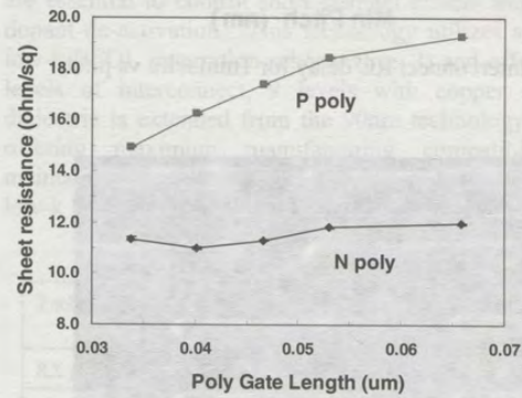
Figure 9: NiSi polycide resistance vs gate size
