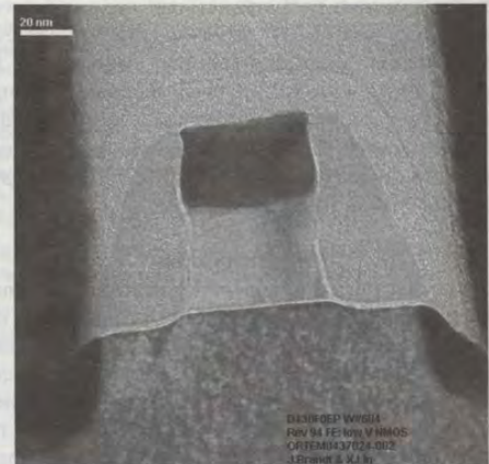
Figure 3: TEM cross section of 35nm NMOS
