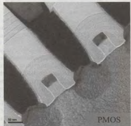
Figure 4: TEM cross section of 35nm PMOS
