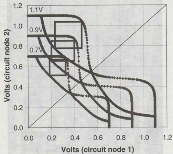
Figure 13: 0.57 \mu\text{m}^2 SRAM cell butterfly curve
