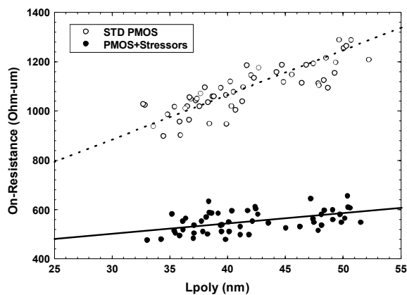
Fig. 6. PMOS on-state resistance measurement constant overdrive vs Lpoly showing mobility and resistance improvement.
