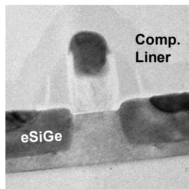
Fig. 2. PMOS with embedded-SiGe and compressive stressed liner on SOI (PMOS stressors).
