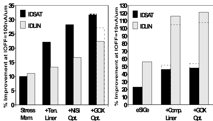
Fig. 8. Percentage NMOS (left) PMOS (right) improvements from Table 2 as individual stress techniques are added. Dotted lines indicate any deviations from the values predicted from Table 2, based on experiments where multiple stress techniques are combined. NMOS stress techniques are fully additive for IDSAT, more than additive for IDLIN with gate oxide optimization. PMOS stress techniques are more than additive for IDSAT, but not fully additive for IDLIN as soon as the compressive liner is added.
