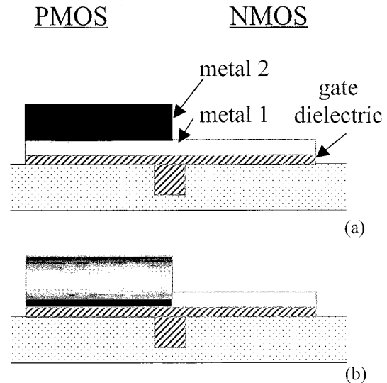
Fig. 1. Schematic illustration of the process flow. (a) CMOS structure after second metal has been removed from the n-MOS side. (b) CMOS structure after annealing shows that the metals on the p-MOS side have interdiffused, and second metal has segregated to the dielectric interface.
