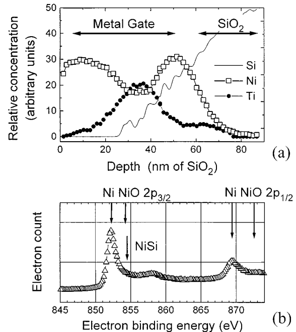
Fig. 4. (a) XPS depth profile for Ti/Ni gate electrode after the 400 °C, 30 min interdiffusion anneal. A large concentration of Ni is present at the \text{SiO}_2 interface, thus Ni determines the gate work function. (b) The photoelectron spectrum taken at the bottom of the MIG electrode shows that only elemental Ni is present at the dielectric interface. This indicates that Ni is thermally stable on \text{SiO}_2 .
