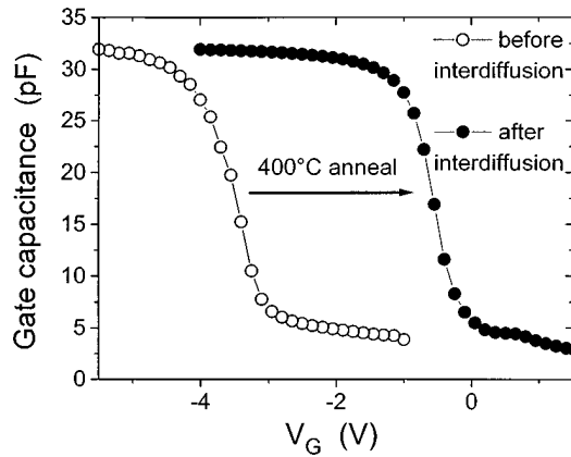
Fig. 2. Capacitance versus voltage characteristics of a fabricated MOS capacitor with Ti/Ni gate. ( t_{\text{ox}} = 35 nm) A large (3 V) shift in the flat-band voltage is due in part to the change in the work function, and in part to the reduction in fixed charge.
