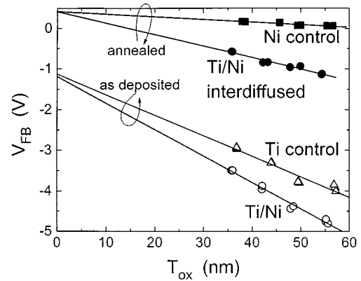
Fig. 3. Before annealing, the work function of the Ti/Ni gate is the same as that of the Ti-control gate; after annealing, it is the same as the work function of the Ni-control gate. As a result of Ni diffusing through Ti to the \text{SiO}_2 interface, the work function of the Ti/Ni gate changes by 1.6 eV.
