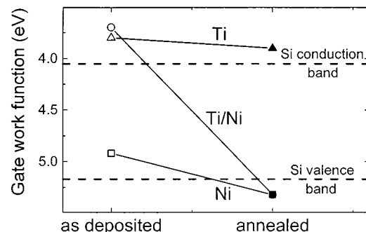
Fig. 5. Work function of Ti is 3.9 \pm 0.08 eV and is appropriate for n-MOS gate application. The work function of the Ti/Ni gate after interdiffusion corresponds to that of Ni ( 5.32 \pm 0.04 eV) and is appropriate for p-MOS gate application.
