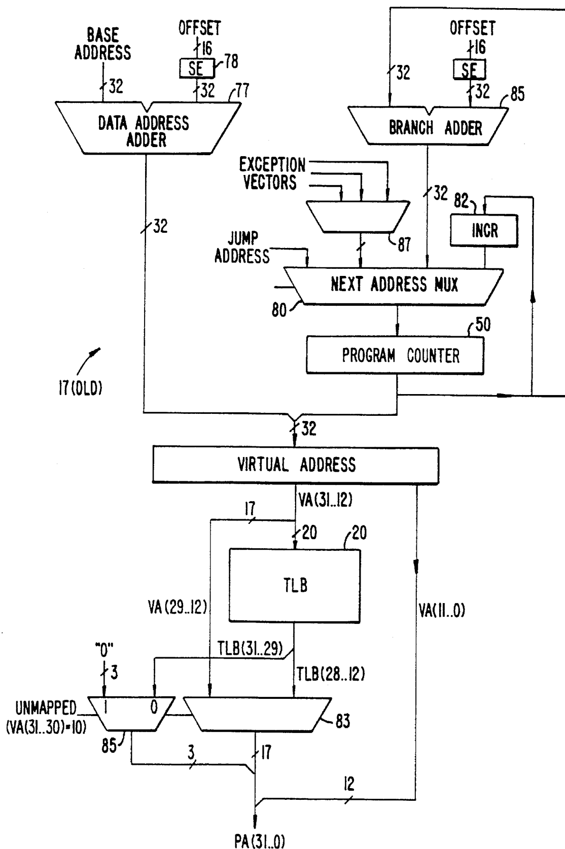
FIG. 3C. (PRIOR ART)
