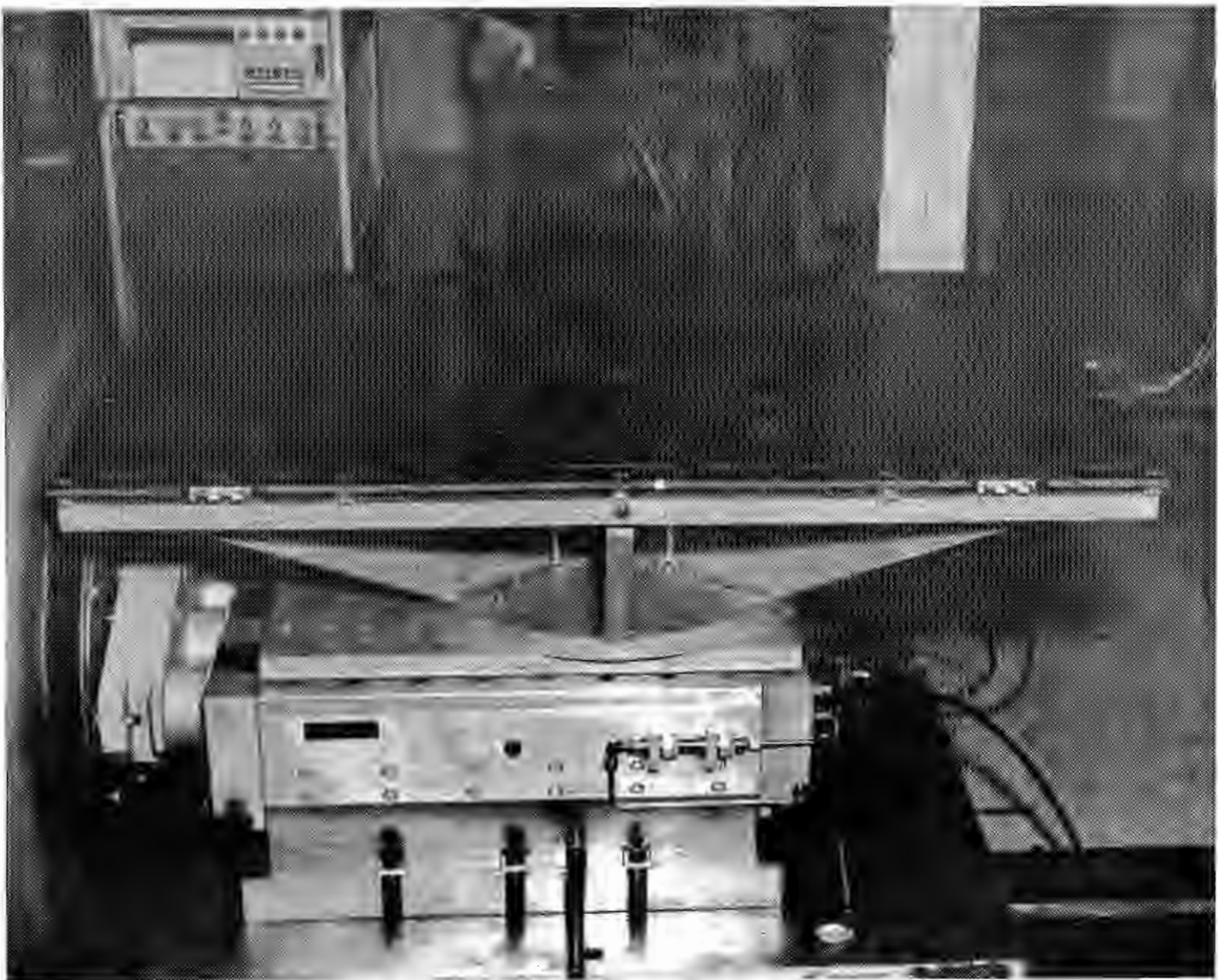
Figure 6.1 Test Setup of Prototype Module for Structural-Dynamic Testing
