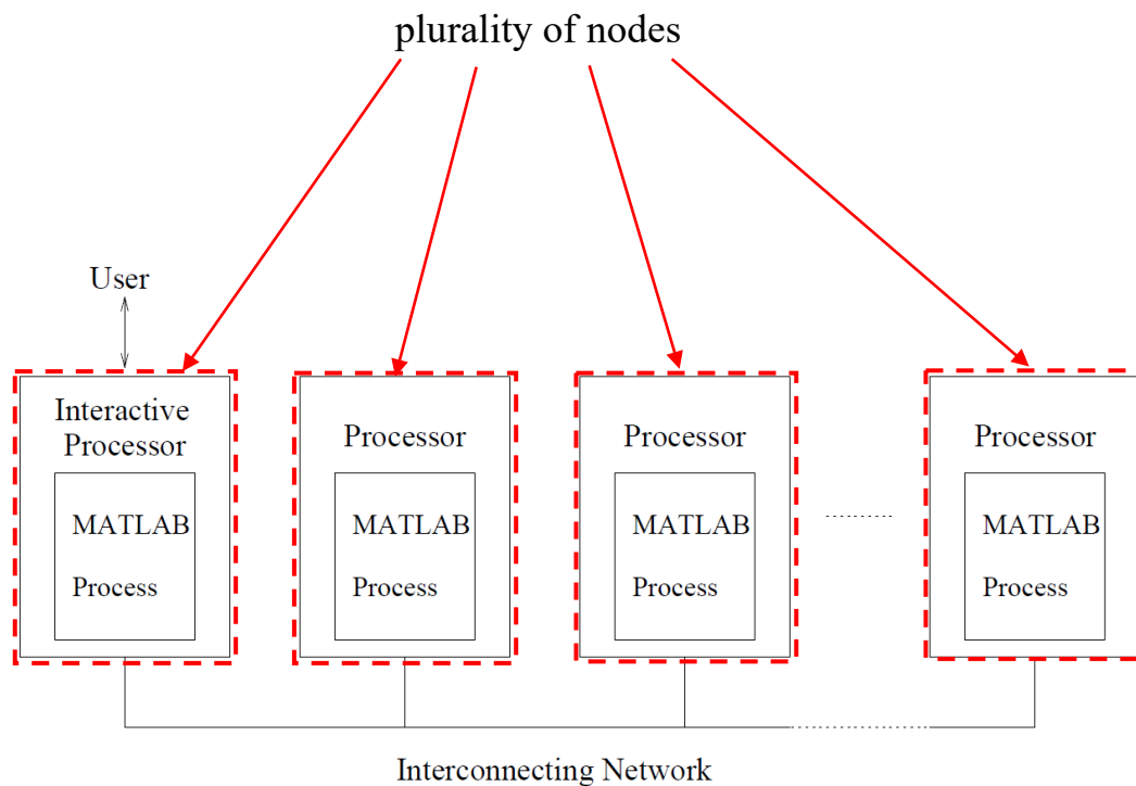
Figure 1: MultiMATLAB Architecture
