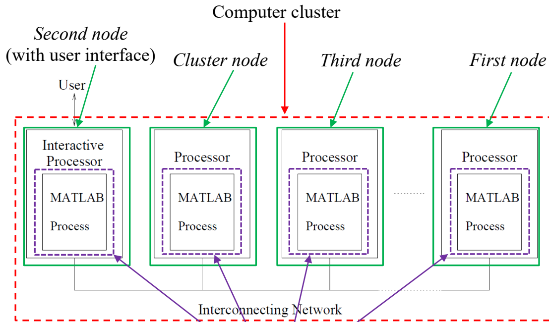
Figure 1: MultiMATLAB Architecture
