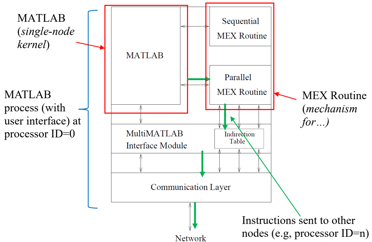
Figure 2: MATLAB Process Addr
