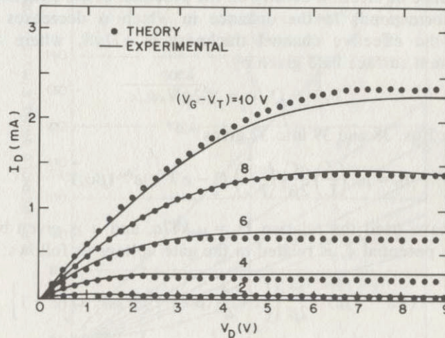
Fig. 10 Theoretical (dots) and experimental (solid lines) drain characteristics of a p-channel MOSFET having d = 2000 \text{ \AA} , N_D = 4.6 \times 10^{14} \text{ cm}^{-3} , and \mu_p = 256 \text{ cm}^2/\text{V-s} . (After Pao and Sah, Ref. 16.)
