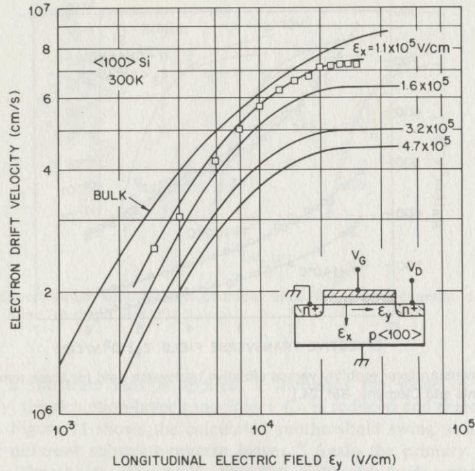
Fig. 14 Electron drift velocity versus longitudinal field for various transverse fields. (After Coen and Muller, Ref. 25; Cooper and Nelson, Ref. 26.)
