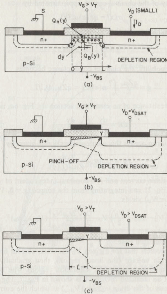
Fig. 6 (a) MOSFET operated in the linear region (low drain voltage). (b) MOSFET operated at onset of saturation. The point Y indicates the pinch-off point. (c) MOSFET operated beyond saturation and the effective channel length is reduced.
