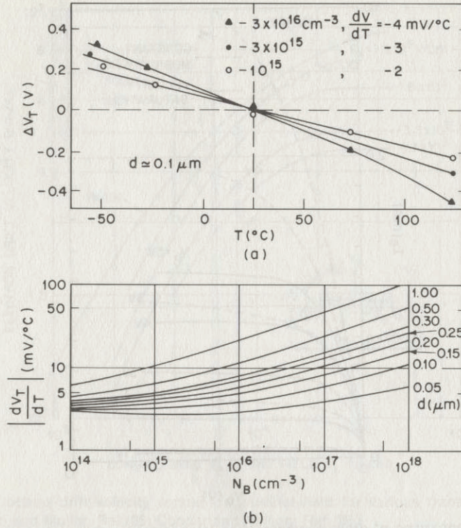
Fig. 16 (a) Experimental measurement of threshold voltage versus temperature. (b) dV_T/dT of a Si-SiO 2 system versus substrate doping with oxide thickness as a parameter. (After Vadasz and Grove, Ref. 29; Wang et al., Ref. 30.)
