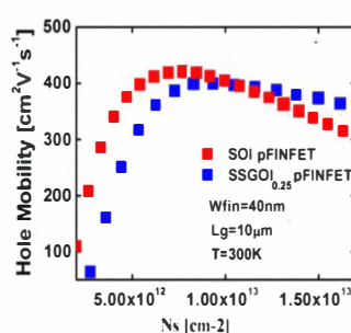
Fig 5. Hole mobility at T=77K in SSGOI 0.25 pFET flattening out at high Ns due to alloy scattering
