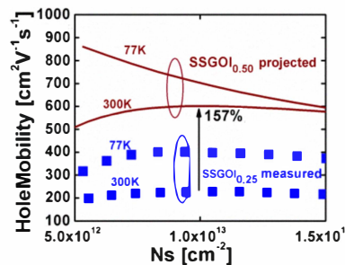
Fig 7. Measured and predicted hole mobilities in SiGe FINFETs
