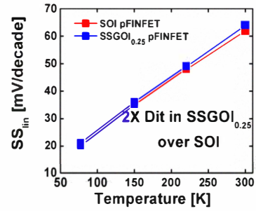
Fig 3. SS lin vs T for SSGOI 0.25 and SOI pFETs
