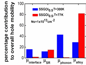
Fig 8. Alloy scattering is the single dominant mechanism at 77K in SSGOI 0.5 FINFET
