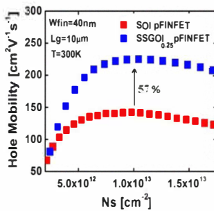
Fig 4. SSGOI 0.25 pFETs shows 57 % improvement in mobility over SOI pFETs
