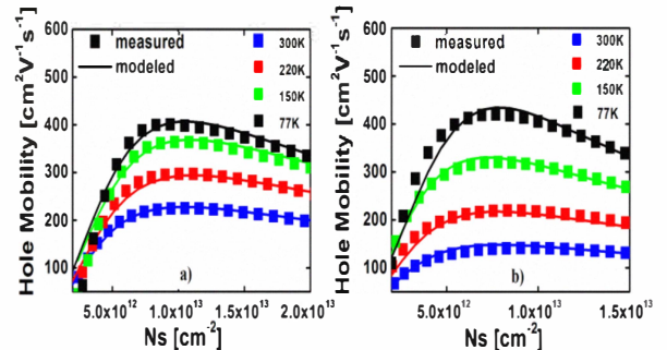
Fig 6. Excellent agreement between modeled and measured mobility values for a) SOI pFET b) SSGOI 0.25 pFET
