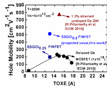
Fig 11. Hole mobility benchmarking as a function of TOXE
