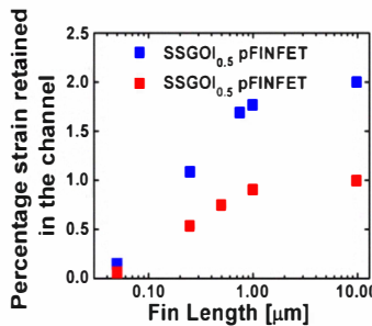
Fig 9. Strain relaxes at the fin edge due to the free surface after patterning
