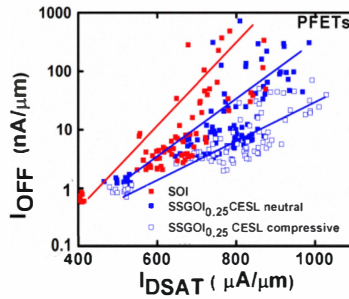
Fig 2. Ioff vs Idsat shows better performance of SSGOI 0.25 over SOI pFETs
