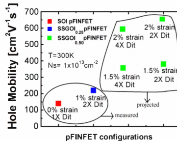
Fig 10. Measured and projected hole mobilities in SiGe FINFETs
