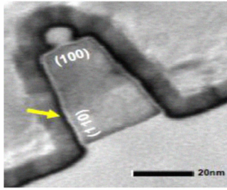
Fig 1. Cross section of SiGe/Si stack fin under gate with Si 0.75 Ge 0.25 (30nm)/Si(10nm)
