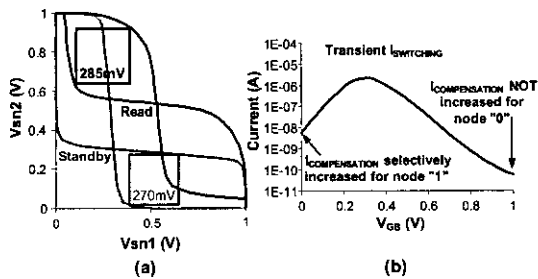
Figure 10. (a) SNM plot for a 4-T cell with feedback during standby (gray) and read (black). (b) Using dynamic feedback, I_{\text{COMPENSATION}} is selectively increased to compensate "1" storage node.
