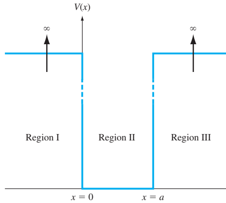
Figure 2.6 | Potential function of the infinite potential well.
