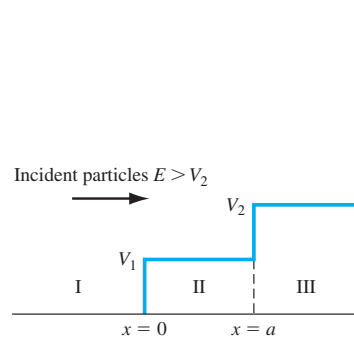
Figure P2.39 | Potential function for Problem 2.39.
