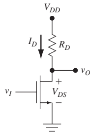
Figure 15.26 | A MOSFET inverter circuit.
