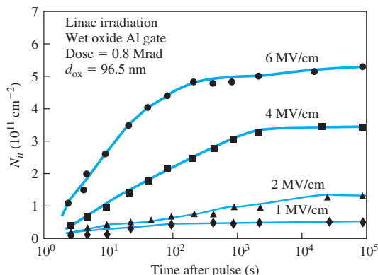
Figure 11.34 | Radiation-induced interface state density versus time after a pulse of ionizing radiation for several values of oxide electric field.
