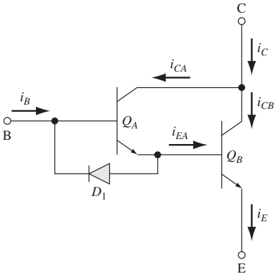
Figure 15.17 | An npn Darlington pair configuration.
