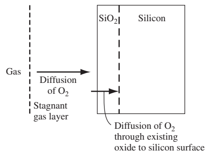
Figure 0.1 | Schematic of the oxidation process.
