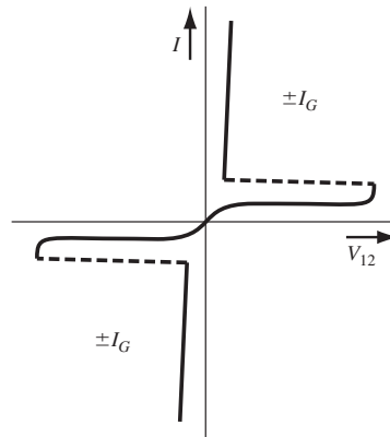
Figure 15.39 | The current–voltage characteristics of the triac.
