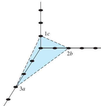
Figure 1.6 | A representative crystal-lattice plane.
