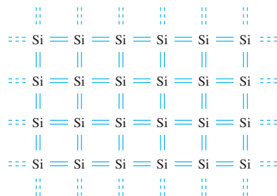
Figure 4.3 | Two-dimensional representation of the intrinsic silicon lattice.
