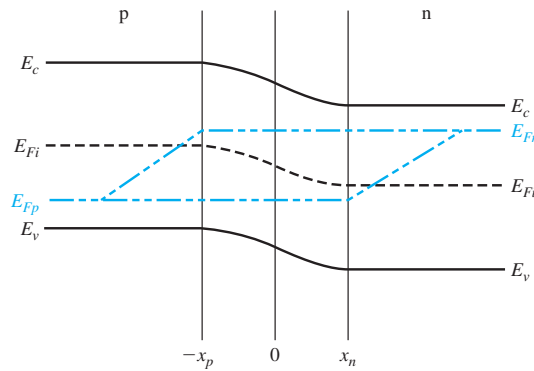
Figure 8.6 | Quasi-Fermi levels through a forward-biased pn junction.
