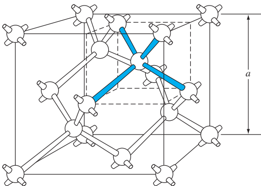
Figure 1.11 | The diamond structure.
