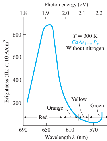
Figure 14.29 | Brightness of GaAsP diodes versus wavelength (or versus bandgap energy). (From Yang [22].)
