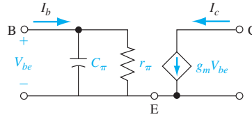
Figure 12.41 | Simplified hybrid-pi equivalent circuit.
