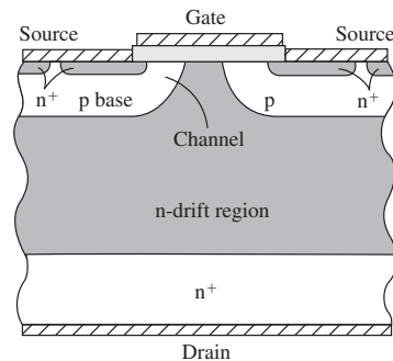
Figure 15.20 | Cross section of a double-diffused MOS (DMOS) transistor.
