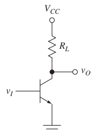
Figure 15.15 | Bipolar common-emitter circuit.
