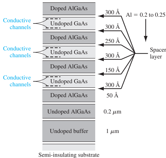
Figure 13.25 | Multilayer modulation-doped heterostructure.
