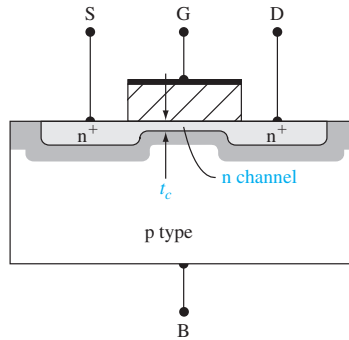
Figure 10.41 | Cross section of an n-channel depletion mode MOSFET.
