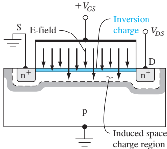
Figure 11.8 | Vertical electric field in an n-channel MOSFET.
