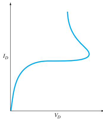
Figure 11.22 | Current-voltage characteristic showing the snapback breakdown effect.
