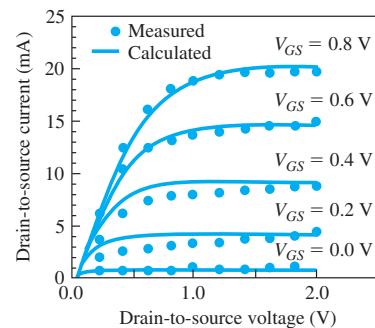
Figure 13.30 | Current–voltage characteristics of an enhancement mode HEMT, in which solid curves are numerical calculations and dots are measured points.
