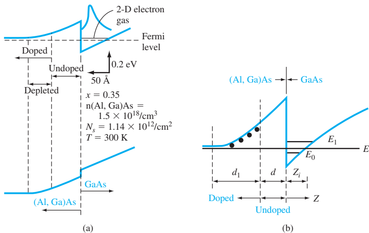
Figure 13.24 | Conduction-band edges for N-AlGaAs–undoped AlGaAs–undoped GaAs heterojunction.
