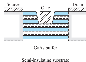
Figure 13.31 | A multilayer HEMT.
