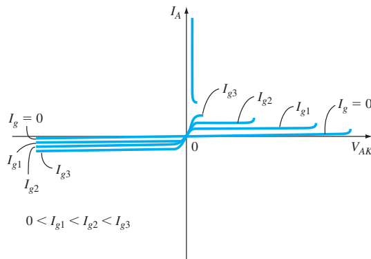
Figure 15.34 | Current–voltage characteristics of an SCR.
