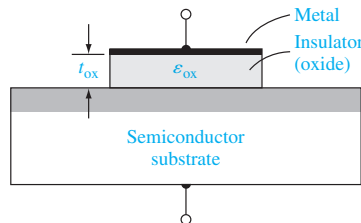
Figure 10.1 | The basic MOS capacitor structure.
