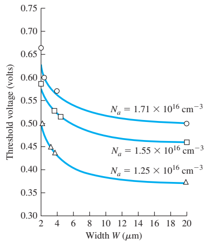
Figure 11.19 | Threshold voltage versus channel width (solid curves, theoretical; points, experimental).
