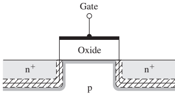
Figure 11.14 | Cross section of a short n-channel MOSFET at flat band.
