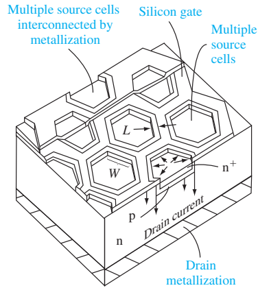
Figure 15.22 | A HEXFET structure.
