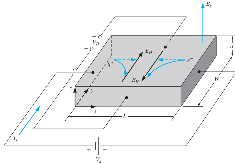
Figure 5.13 | Geometry for measuring the Hall effect.
