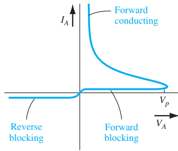
Figure 15.32 | The current–voltage characteristics of the pnpn device.
