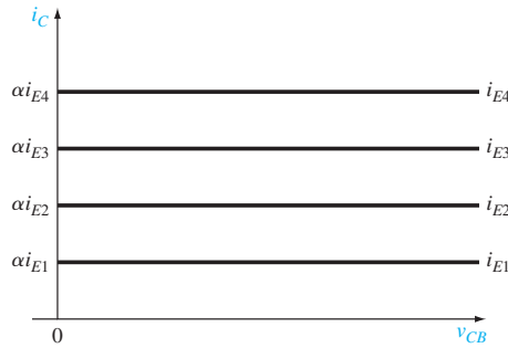
Figure 12.7 | Ideal bipolar transistor common-base current–voltage characteristics.
