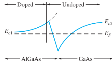
Figure 9.22 | Conduction-band edge at a graded heterojunction.
