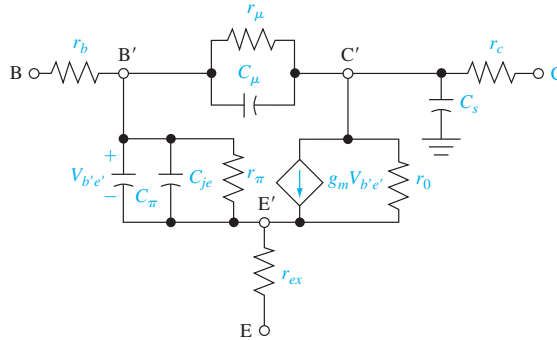
Figure 12.40 | Hybrid-pi equivalent circuit.
