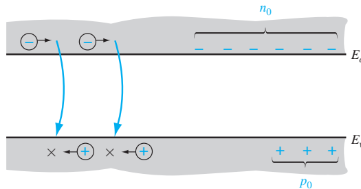
Figure 6.3 | Recombination of excess carriers reestablishing thermal equilibrium.
