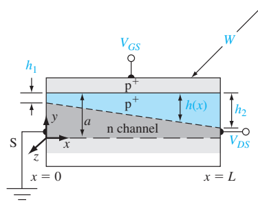
Figure 13.11 | Simplified geometry of an n-channel pn JFET.
