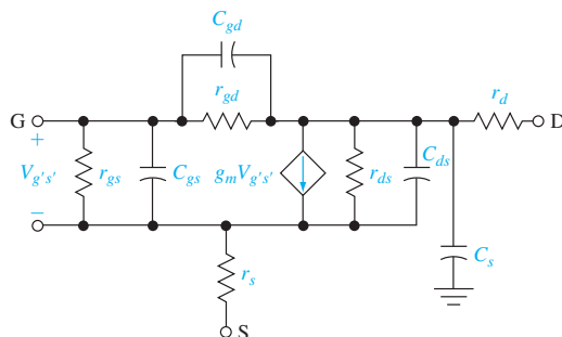
Figure 13.19 | Small-signal equivalent circuit of JFET.
