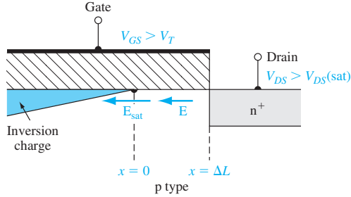
Figure 11.6 | Expanded view of cross section near the drain terminal of an n-channel MOSFET showing the channel length modulation effect.
