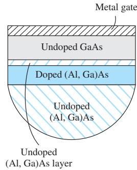
Figure 13.27 | An “inverted” GaAs–AlGaAs HEMT. (From Shur [13].)
