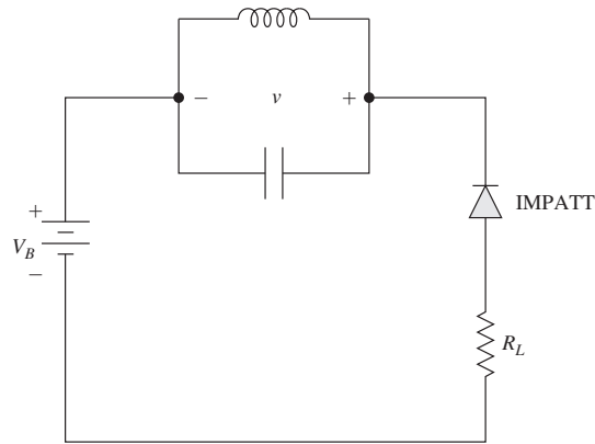
Figure 15.9 | Circuit for an IMPATT diode oscillator.
