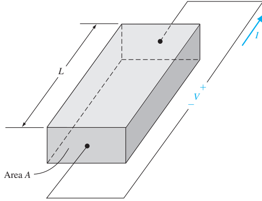
Figure 5.5 | Bar of semiconductor material as a resistor.
