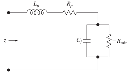
Figure 15.2 | Equivalent circuit of the tunnel diode.
