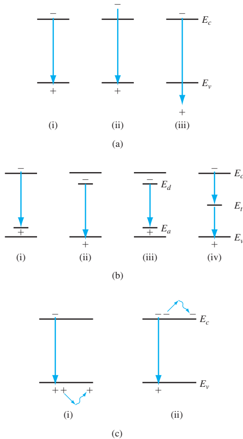
Figure 14.21 | Basic transitions in a semiconductor.
