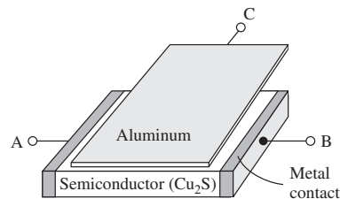
Figure 13.1 | Idealization of the Lilienfeld transistor. (From Pierret [10].)
