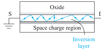
Figure 11.9 | Schematic of carrier surface scattering effects.
