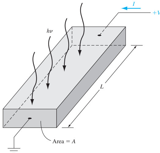
Figure 14.16 | A photoconductor.
