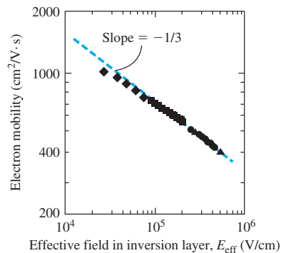
Figure 11.10 | Measured inversion layer electron mobility versus electric field at the inversion layer.
