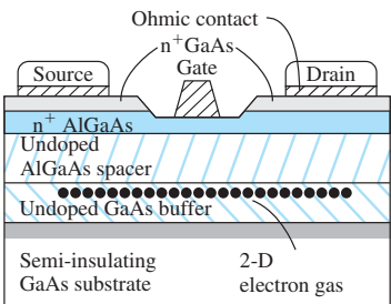
Figure 13.26 | A “normal” AlGaAs–GaAs HEMT.
