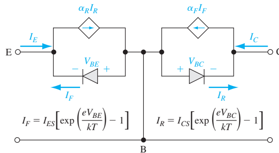
Figure 12.37 | Basic Ebers–Moll equivalent circuit.
