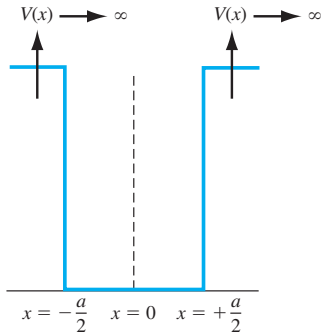
Figure P2.29 | Potential function for Problem 2.29.
