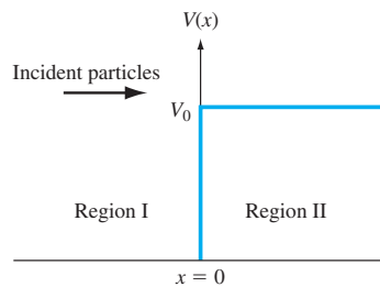
Figure 2.8 | The step potential function.
