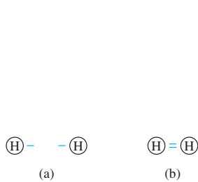
Figure 1.16 | Representation of (a) hydrogen valence electrons and (b) covalent bonding in a hydrogen molecule.
