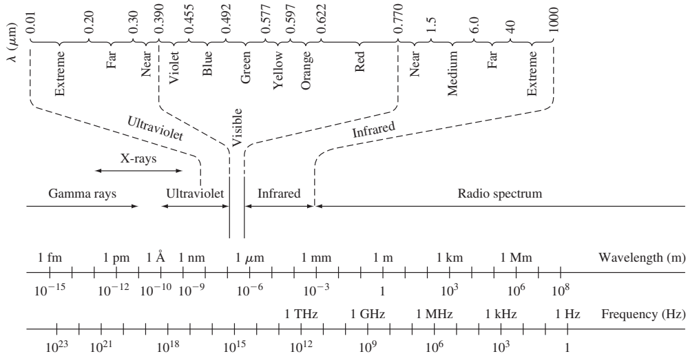
Figure 2.4 | The electromagnetic frequency spectrum.
