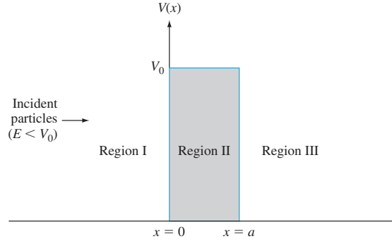
Figure 2.9 | The potential barrier function.
