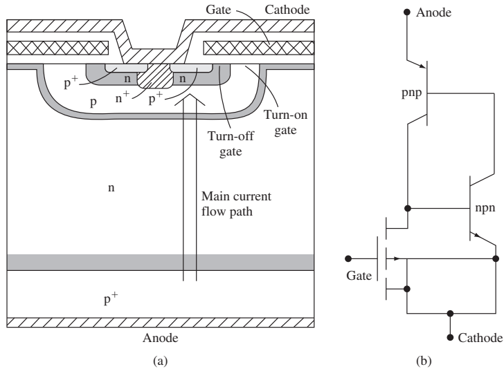
Figure 15.41 | (a) The MOS turn-off thyristor. (b) Equivalent circuit for the MOS turn-off thyristor.
