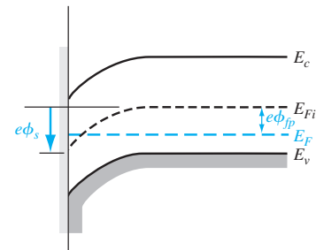
Figure 11.2 | Energy-band diagram when \phi_{fp} < \phi_s < 2\phi_{fp} .
