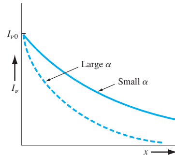
Figure 14.3 | Photon intensity versus distance for two absorption coefficients.
