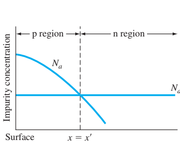
Figure 7.16 | Impurity concentrations of a pn junction with a nonuniformly doped p region.
