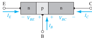
Figure 12.36 | Current direction and voltage polarity definitions for the Ebers–Moll model.
