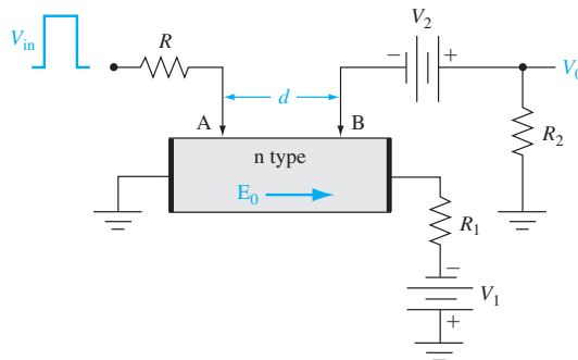
Figure 6.11 | The basic Haynes–Shockley experimental arrangement.
