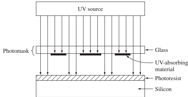
Figure 0.2 | Schematic showing the use of a photomask.
