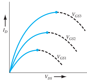
Figure 10.47 | Plots of I_D versus V_{DS} from Equation (10.62).
