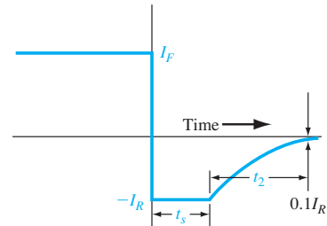
Figure 8.26 | Current characteristic versus time during diode switching.
