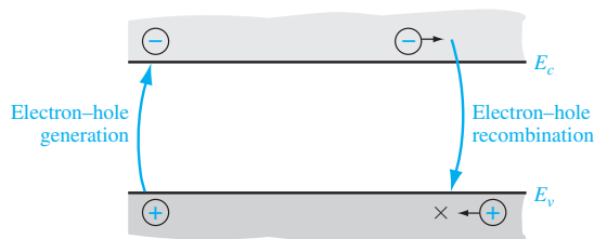
Figure 6.1 | Electron-hole generation and recombination.
