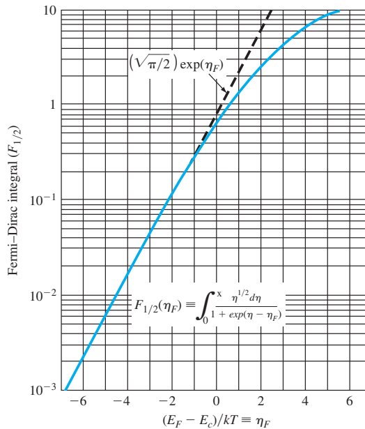
Figure 4.10 | The Fermi–Dirac integral F_{1/2} as a function of the Fermi energy.
