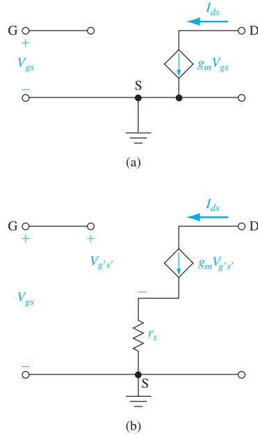
Figure 13.20 | (a) Ideal low-frequency small-signal equivalent circuit. (b) Ideal equivalent circuit including r_s .
