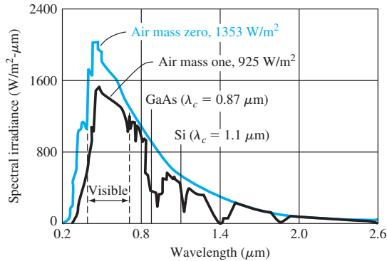
Figure 14.9 | Solar spectral irradiance. (From Sze [18].)
