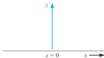
Figure 6.6 | Steady-state generation rate at x = 0 .
