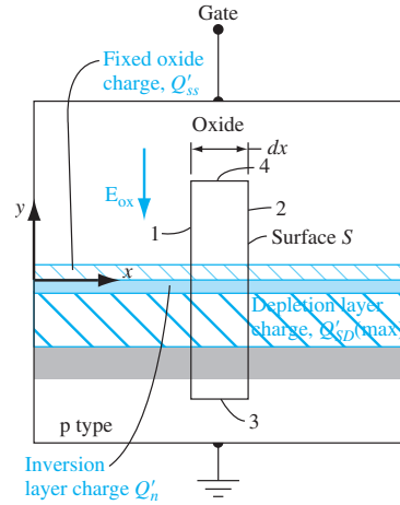
Figure 10.45 | Geometry for applying Gauss's law.
