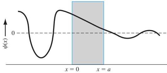
Figure 2.10 | The wave functions through the potential barrier.
