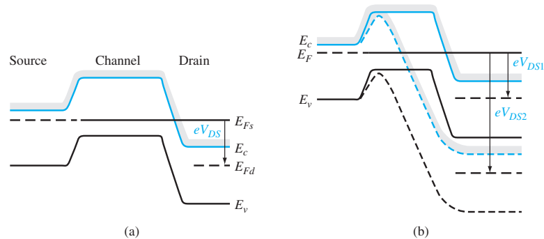
Figure 11.25 | (a) Equipotential plot along the surface of a long-channel MOSFET. (b) Equipotential plot along the surface of a short-channel MOSFET before and after punch-through.
