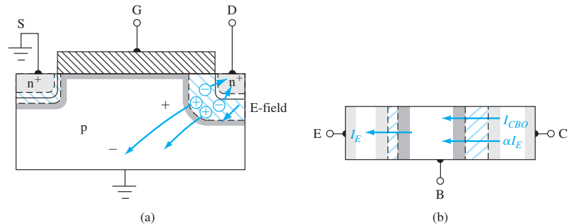
Figure 11.24 | (a) Substrate current–induced voltage drop caused by avalanche multiplication at the drain. (b) Currents in the parasitic bipolar transistor.
