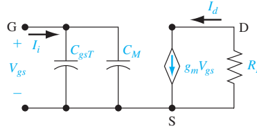
Figure 10.57 | Small-signal equivalent circuit including Miller capacitance.
