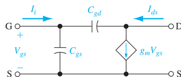
Figure 13.22 | A small-signal equivalent circuit with capacitance.
