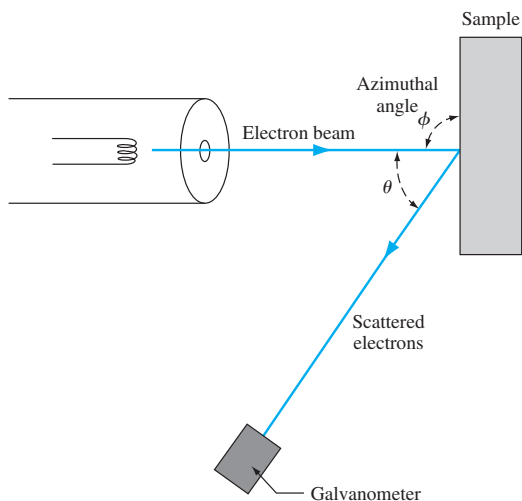
Figure 2.2 | Experimental arrangement of the Davisson–Germer experiment.
