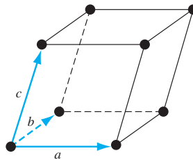
Figure 1.4 | A generalized primitive unit cell.
