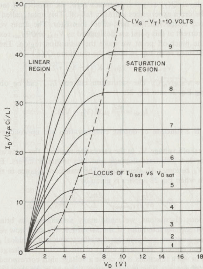
Fig. 7 Idealized drain characteristics ( I_D versus V_D ) of a MOSFET. The dashed line indicates the locus of the saturation drain voltage ( V_{D sat} ). For V_D > V_{D sat} , the drain current remains constant.
