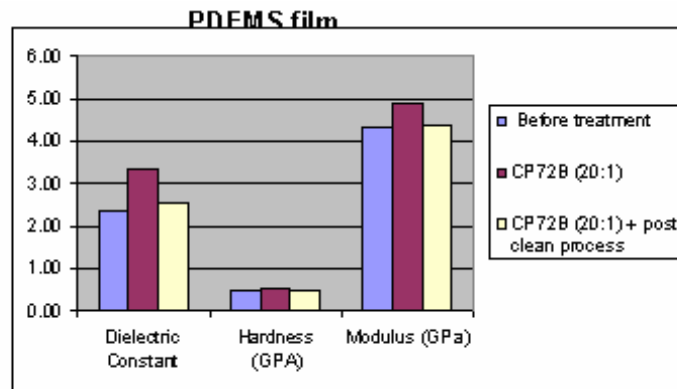
Figure 13: Effect of CoppeReady® CP72B on PDEMS Film[15]
