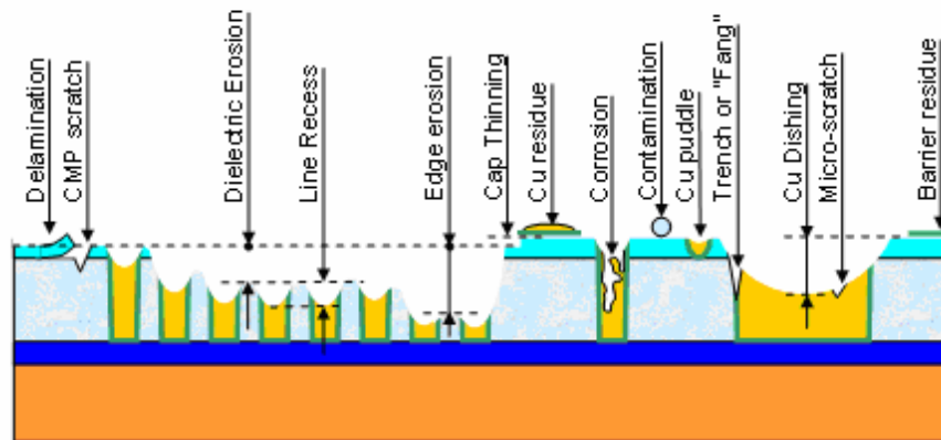
Figure 4: Basic failure modes for Cu CMP
