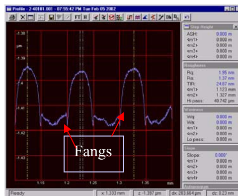
Figure 10: Atomic Force Profile of a pattern wafer (MIT 854) after barrier CMP showing fang formation in the trenches [13].
