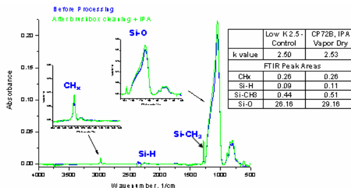
Figure 15: FTIR Spectra of CoppeReady® CP72B on PDEMS® ( k=2.5 )
