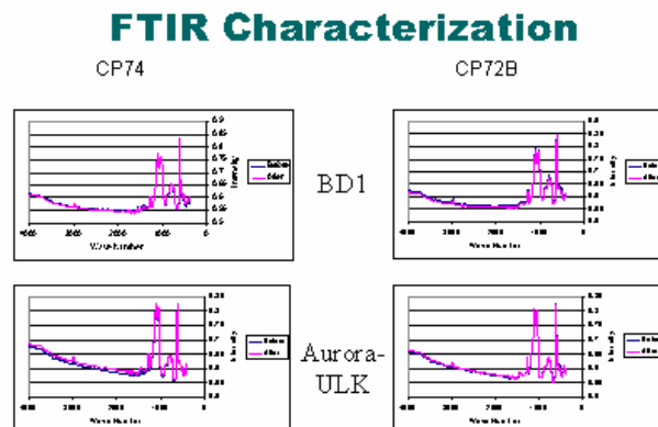
Figure 12: No Damage to Dielectric Films after post CMP Cleaning[14]
