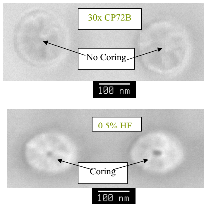
Figure 8: SEM images of plug structures processed with different chemistries
