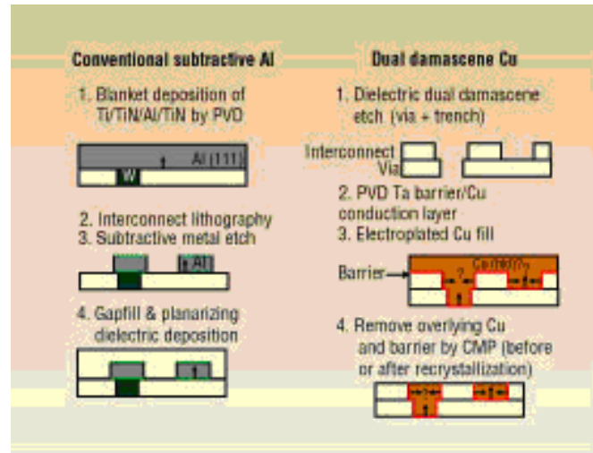
Figure 3: Comparison between conventional Al interconnect and Cu dual damascene
