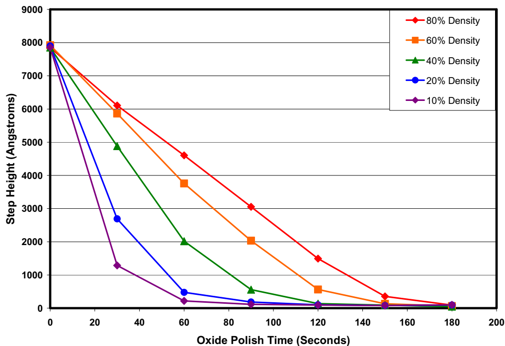
Figure 6. Step height as a function of oxide CMP polish time for structures with differing pattern densities.
