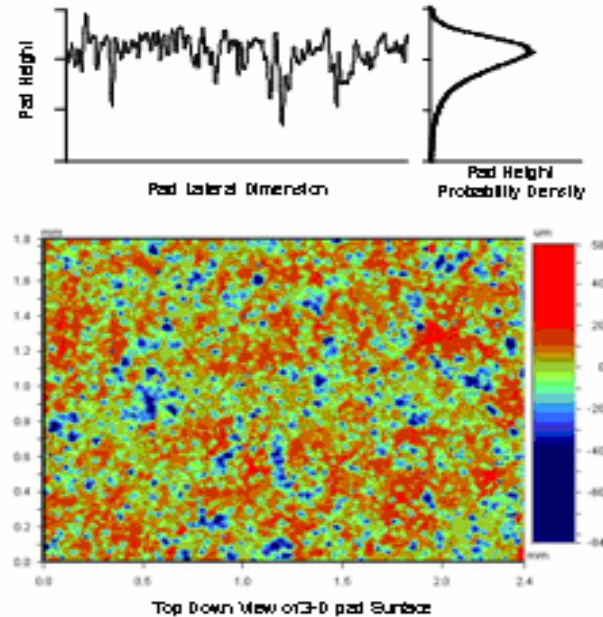
Figure 7: Pad Asperities [9]
