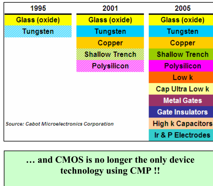
Figure 1: Various film stacks polished using CMP in CMOS Technology
