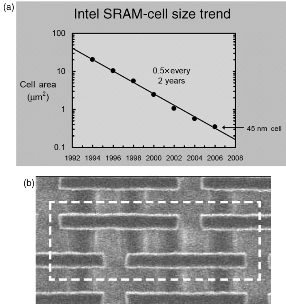
FIGURE 17: SRAM-cell size is a key metric of scaling for microprocessor technologies. Intel Corp. maintains a 50% aerial shrink of SRAM cell with each technology - (a). 45-nm technology SRAM cell (b) is the latest addition to the trend. The dotted line represents the six transistor cell—horizontal lines are the MOS gates and the vertical lines are diffusion regions
