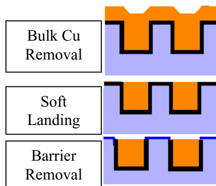
Figure 9: Schematic representation of 3 key steps in the modern Cu-CMP process.
