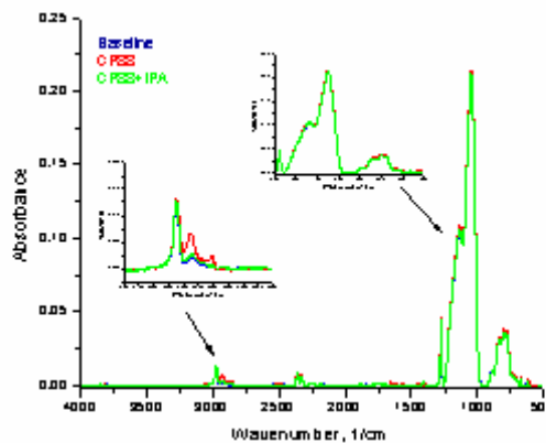
Figure 16: FTIR Spectra of CoppeReady® CP72B on PDEMS® ( k=2.2 )
