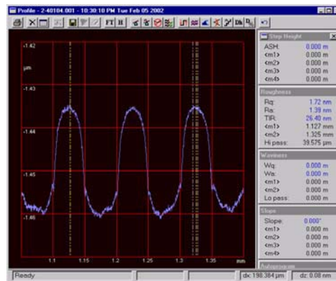
Figure 11: Atomic Force Profile of a pattern wafer (MIT 854) after barrier CMP, showing no fang formation in the trenches [13].
