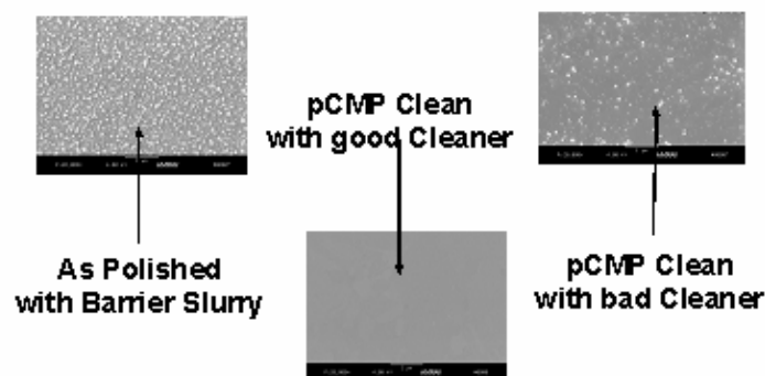
Figure 14: Post CMP cleaning performance comparison on Cu wafers[17]
