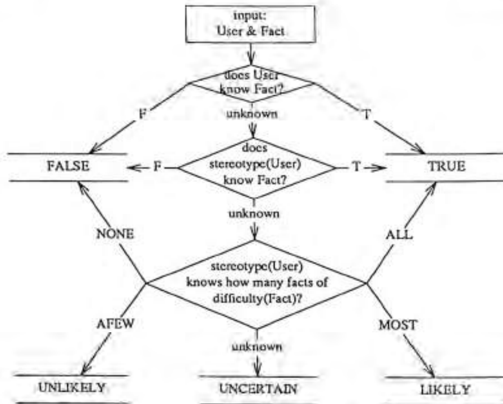
Figure 4. Algorithm for determining whether User knows Fact
