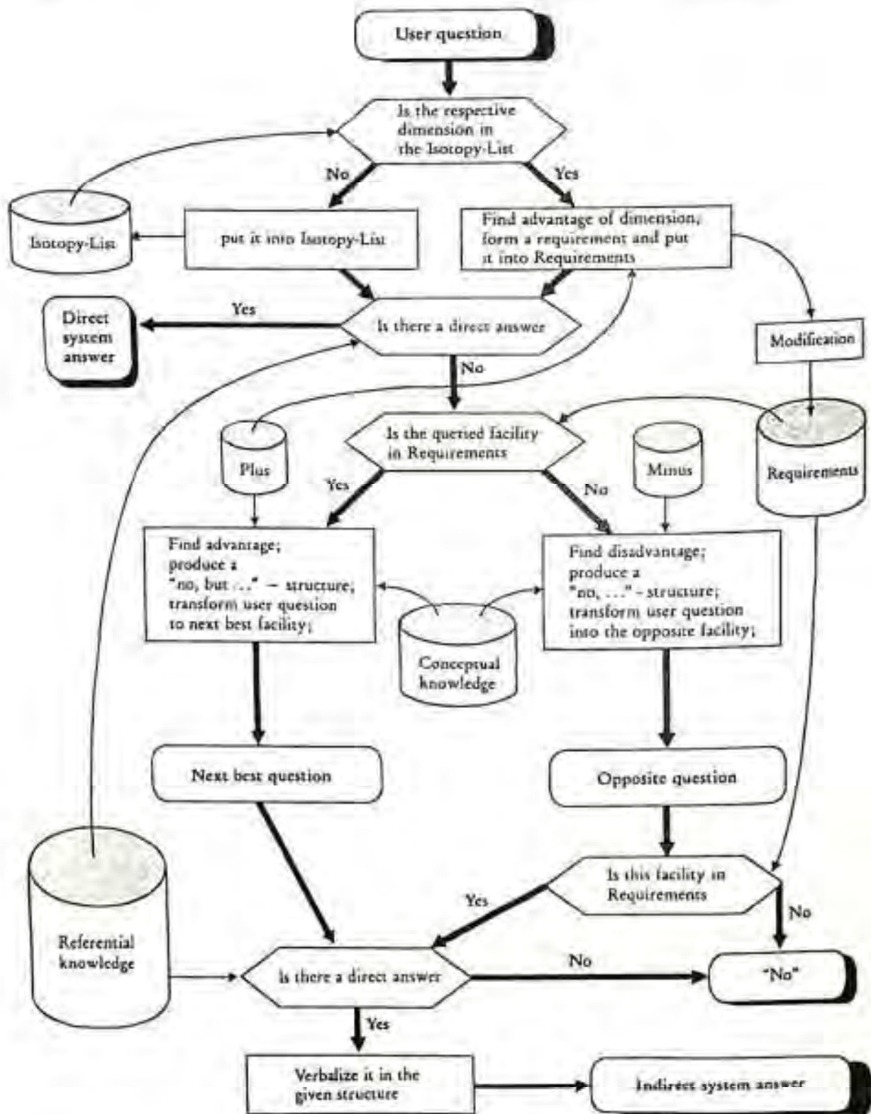
Figure 4. Overanswering using evaluation standards and isotopy
