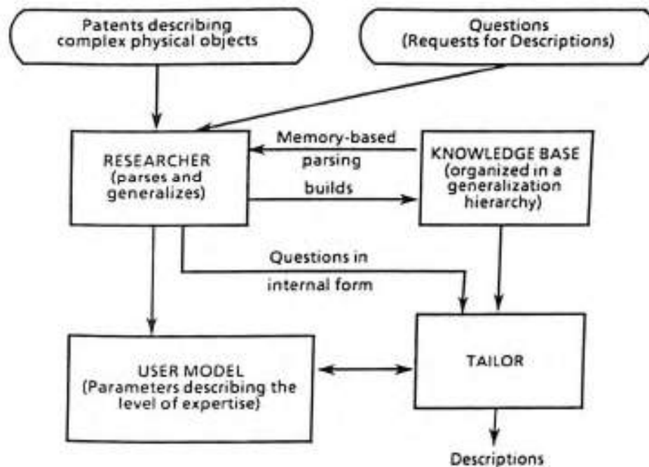
Figure 12. RESEARCHER and the TAILOR system
