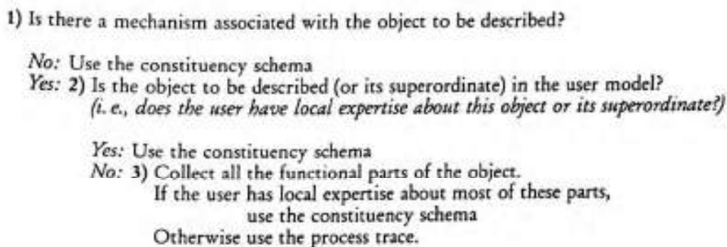
Figure 7. The decision algorithm for the initial strategy
