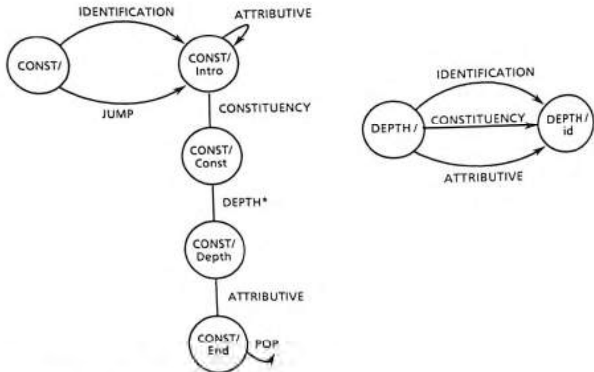
Figure 14. The constituency schema
