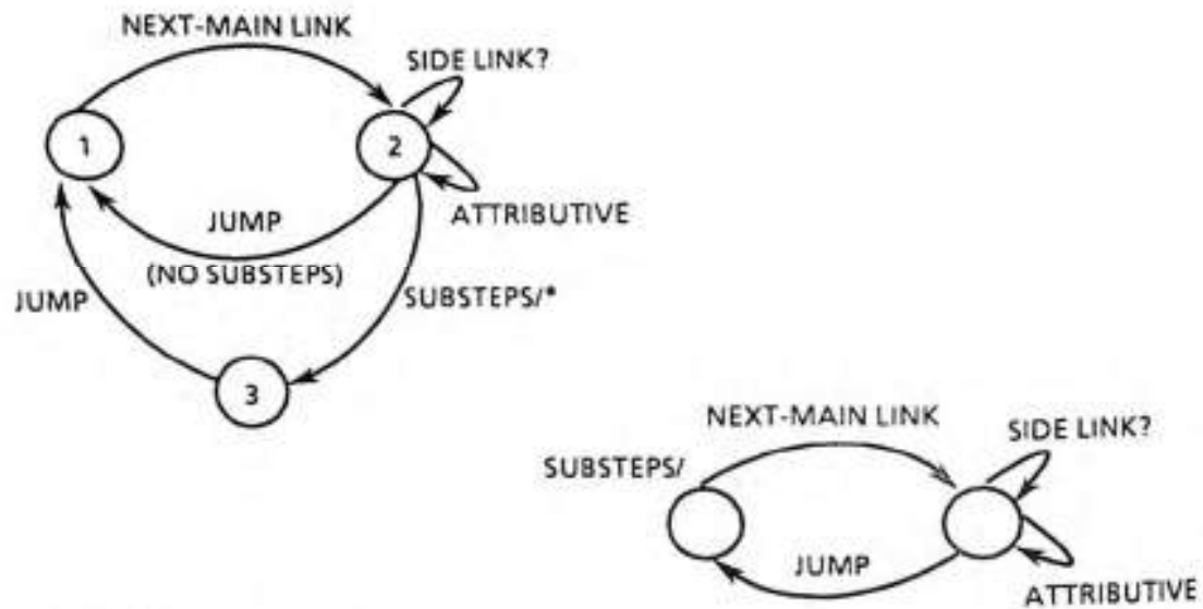
Figure 16. The process trace
