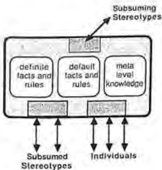
Figure 5. A stereotype
