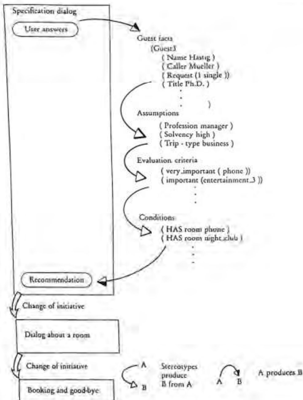
Figure 2. Modeling user's wants in HAM-ANS
