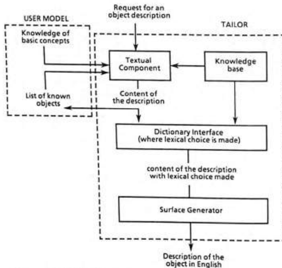
Figure 13. The TAILOR system
