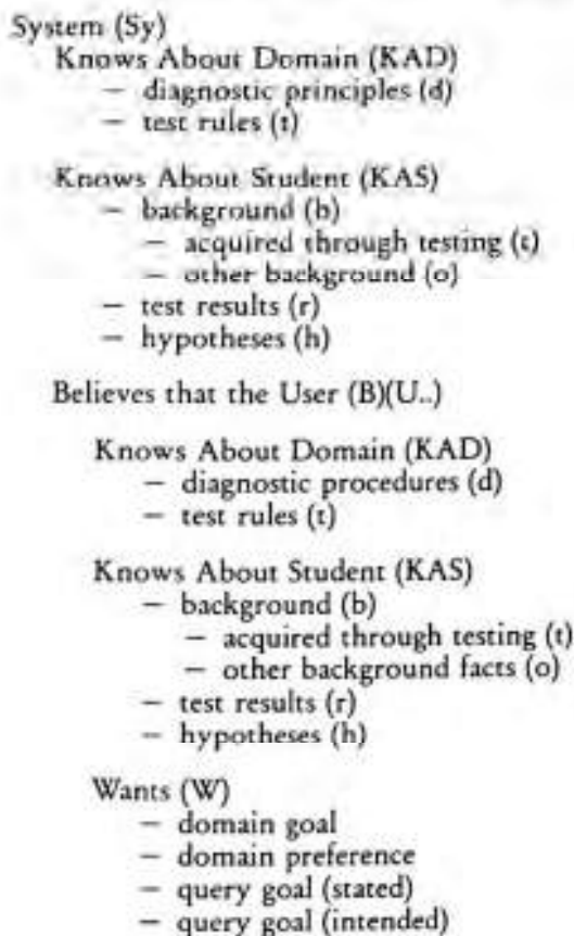
Figure 1. Labeling of system knowledge bases
