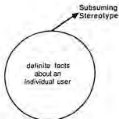
Figure 6. An individual
