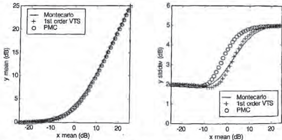
Figure 10.35 Means and standard deviation of noisy log-spectrum y in dB according to Eq. (10.165). The distribution of the noise log-spectrum n is Gaussian with mean 0 dB and standard deviation 2 dB. The distribution of the clean log-spectrum x is Gaussian with a standard deviation of 5 dB and a mean varying from -25 dB to 25 dB. The mean of y is well estimated in both PMC and first-order VTS. The standard deviation of y is more accurate in first-order VTS than in PMC.
