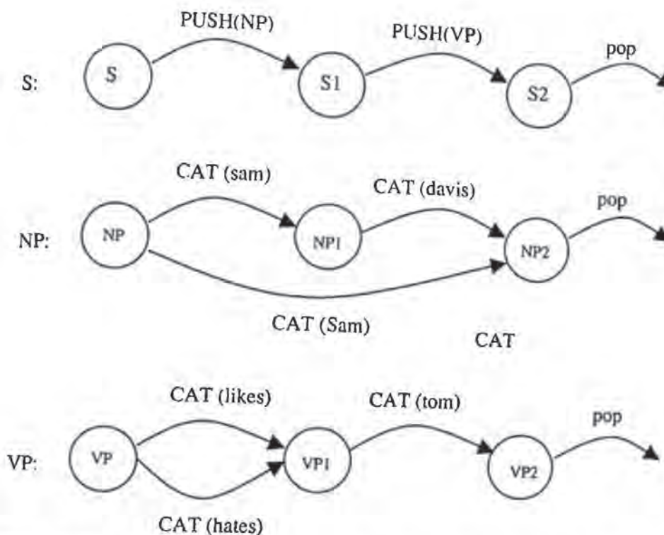
Figure 12.13 A simple RTN example with three types of arcs: CAT(x) , PUSH(x) , POP .
