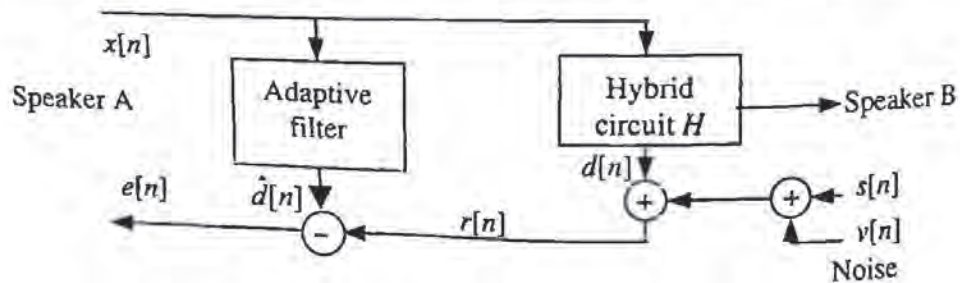
Figure 10.18 Block diagram of echo canceling for a telephone communication. x[n] represents the remote call signal, s[n] the local outgoing signal. The hybrid circuit H does a 2-4 wire conversion and is nonideal because of impedance mismatches.
