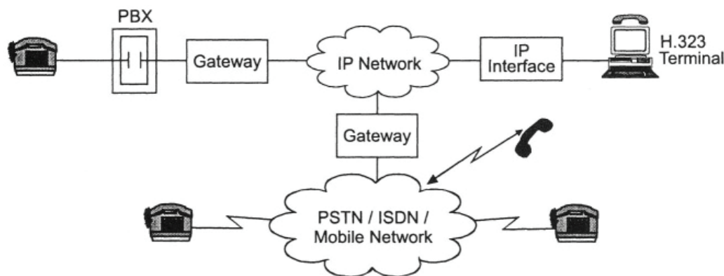
Figure 2.3. Interconnection of a mixed PSTN/ISDN/mobile network with an IP-based network, terminated with wireless or wireline telephones, an H.323 terminal, and a PBX, see ITU-T Rec. G.108(1999).
