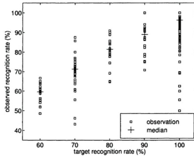
Figure 6.10. Comparison of observed and target recognition rates for the recognizer simulation in experiment 6.3.
