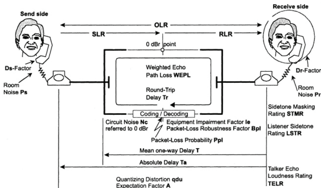
Figure 2.10. Reference connection for network planning purposes, see ITU-T Rec. G.107 (2003).
