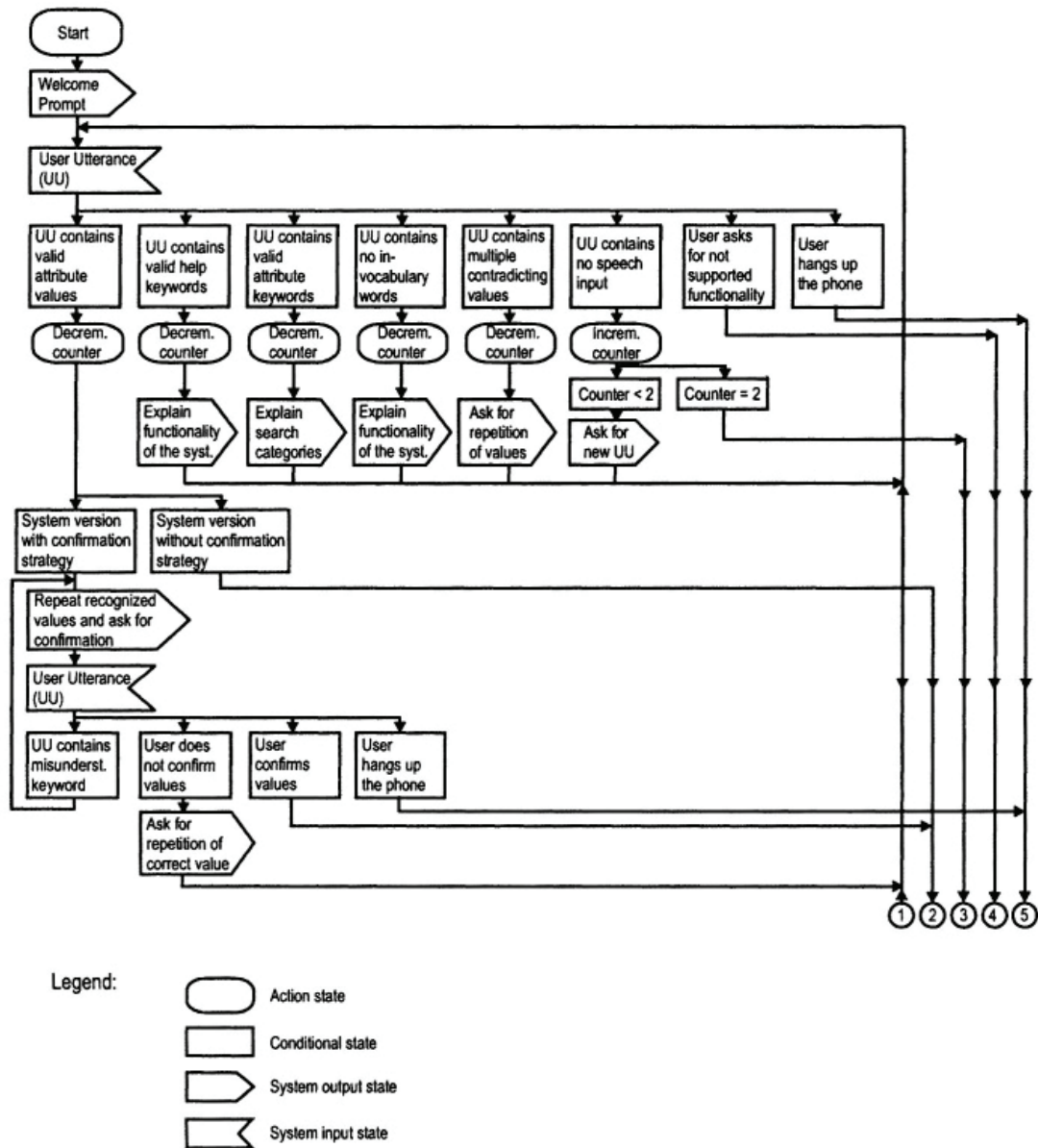
Figure C. 1. Dialogue flow in the BoRIS restaurant information system of experiment 6.3, part 1.
