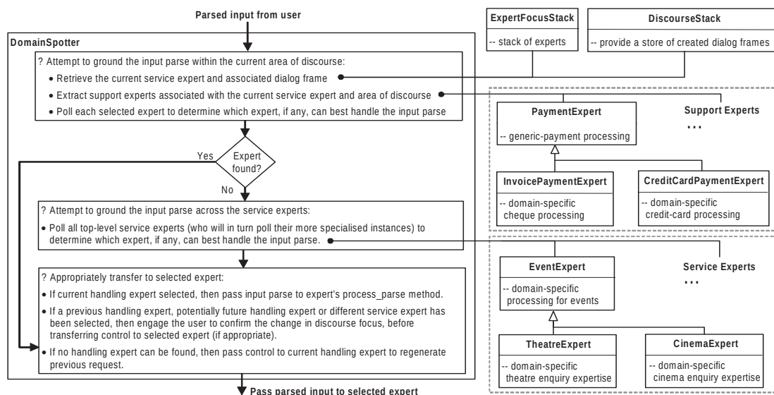
Figure 1: Domain spotting to further an on-going transaction
