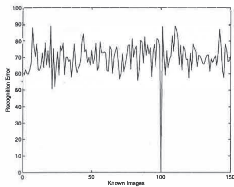
Fig. 6. Recognition result for a known input face image (number 100).
