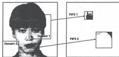
Fig. 3. Partitioned iterated function systems.
