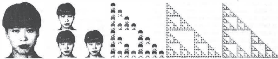
Fig. 2. An attractor of an IFS with three maps.
