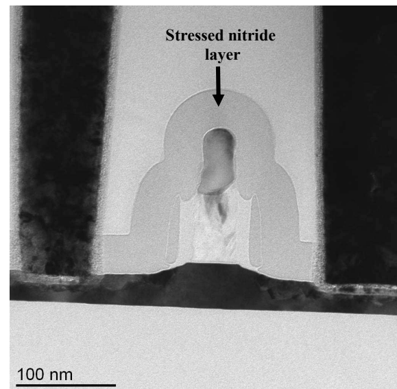
Figure 8. NMOS Transistor in IBM PPC970FX
