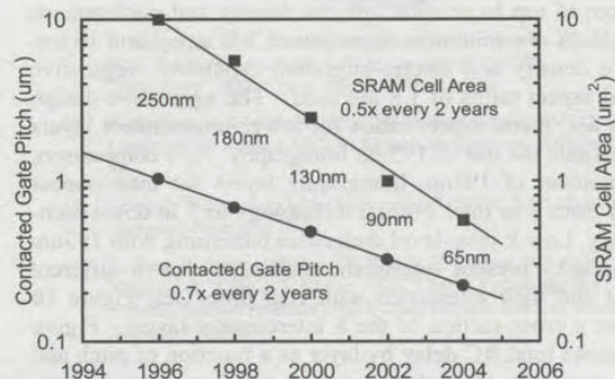
Figure 1: Intel contacted gate pitch and SRAM area trends
