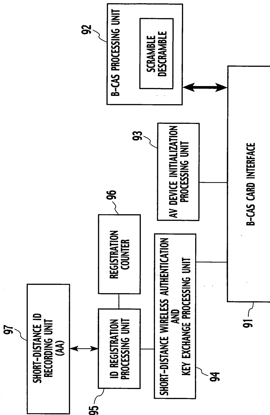
FIG.26 INTERNAL FEATURES OF B-CAS CARD
