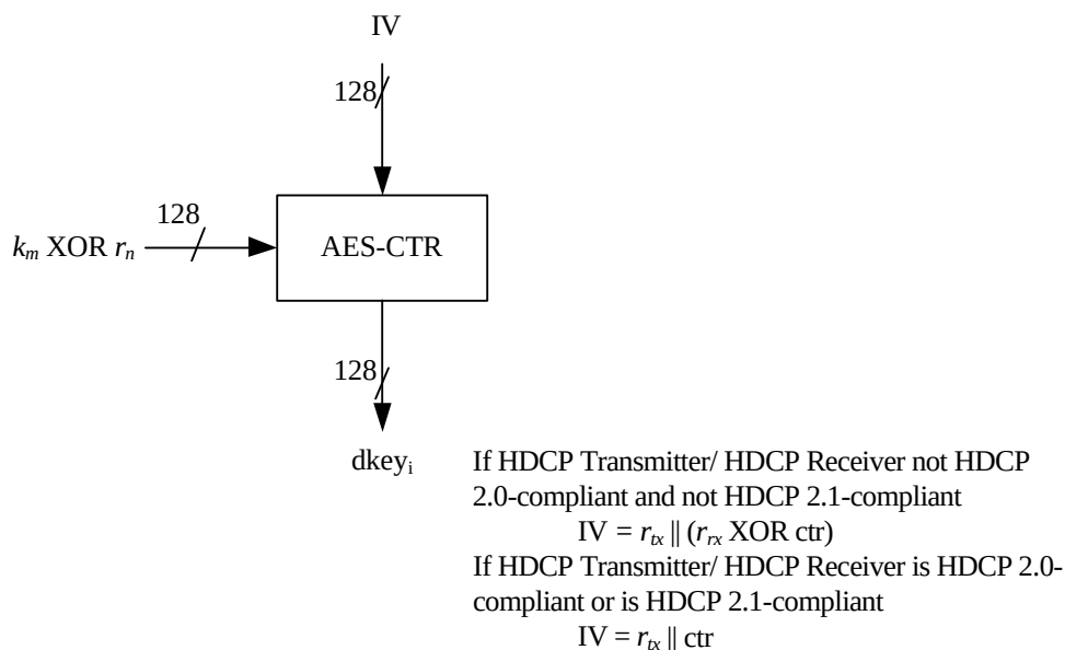
Figure 2.11. Key Derivation
