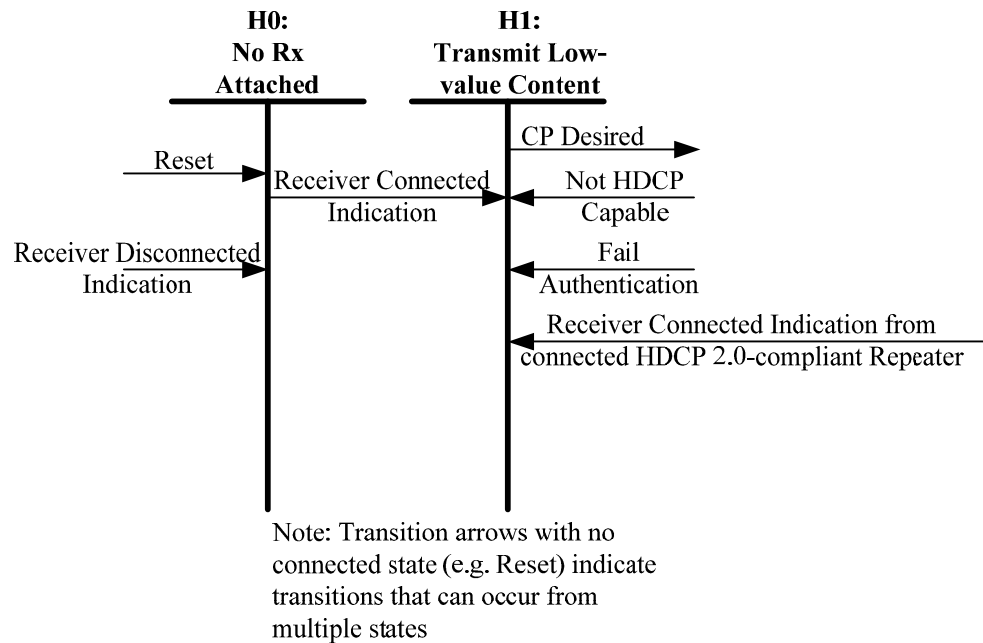
Figure 2.12. HDCP Transmitter Link State Diagram
