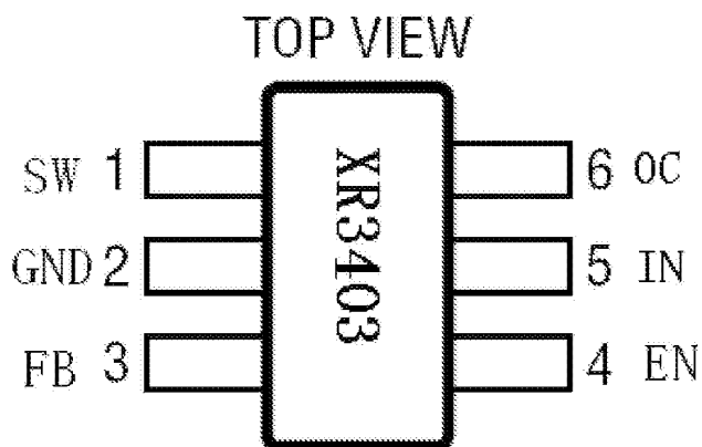
Figure 2. PIN Configuration
