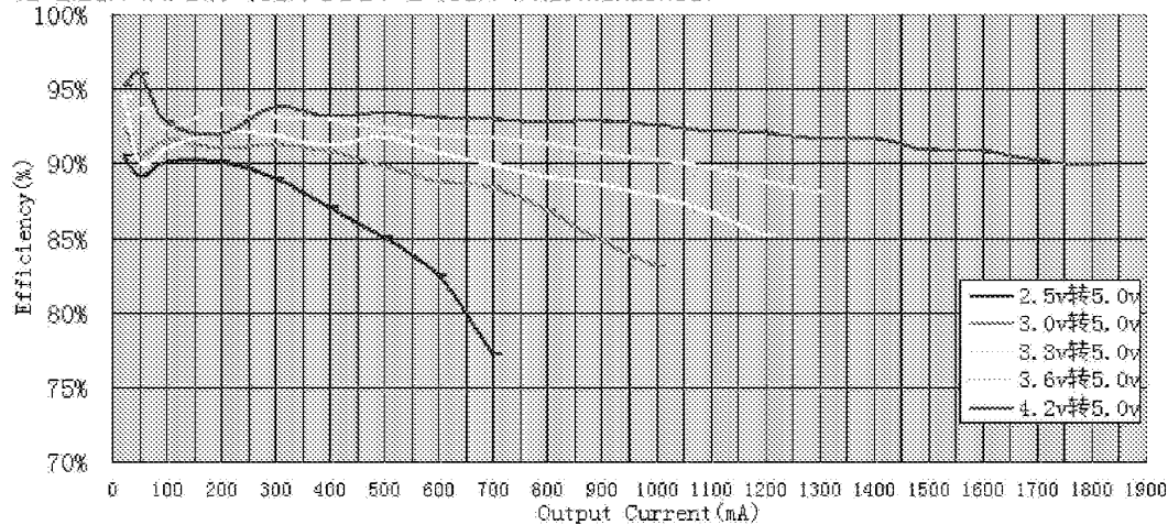
Efficiency vs. Output Current (Vout=5V Rset=300K)
