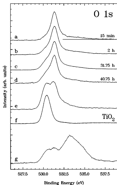
FIG. 3. The O 1s signals, shown in curves a – d , exhibit a prominent shoulder at the low binding energy side which increases with the degree of oxidation of the sample surface. Curve e shows the O 1s signal after the sample was subjected to atmospheric conditions. The O 1s signal of TiO 2 is presented in curve f for comparison.
