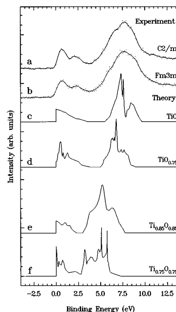
FIG. 10. Comparison of the experimental valence band DOS with those obtained by some of the latest band structure calculations for different model structures (Refs. 10, 19, and 20).
