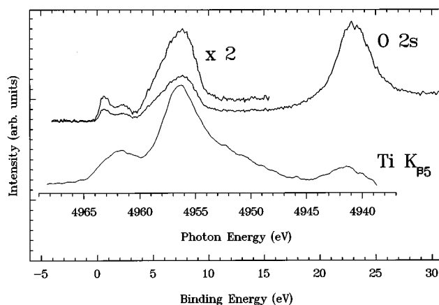
FIG. 7. Distribution of the Ti 4p partial DOS in the valence band region. The Ti K_{\beta 5} x-ray emission spectrum reveals a hybridization of Ti 4p and O 2s states.
