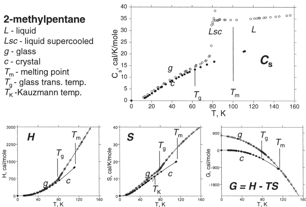
Fig. 2. Thermodynamic properties of the crystalline and amorphous phases of 2-methylpentane. The heat capacity ( C_p ) data (Douslin, D. R.; Huffman, H. M. J. Am. Chem. Soc. 1946 , 68, 173) have been integrated to give the enthalpy ( H ), entropy ( S ), and free energy ( G ). Excess properties correspond to the difference between the crystalline and amorphous lines. The “entropy crisis” of Kauzmann (Kauzmann, W. Chem. Rev. 1948 , 43, 219–256) is seen in the S panel as the impending crossing of the liquid line with the crystal line as the temperature decreases below the crystal melting point T_m . If not for the intervention of the glass transition at T_g , the liquid line would have crossed the crystal line at T_K . This would be an absurdity, since the liquid entropy would be lower than crystal entropy below T_K .
