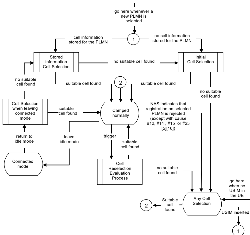
Figure 5.2.2-2: RRC_IDLE Cell Selection and Reselection for NB-IoT
