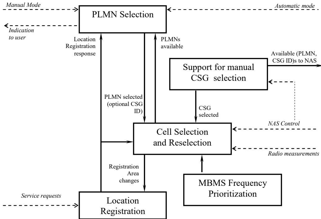
Figure 4.1-1: Overall Idle Mode process
