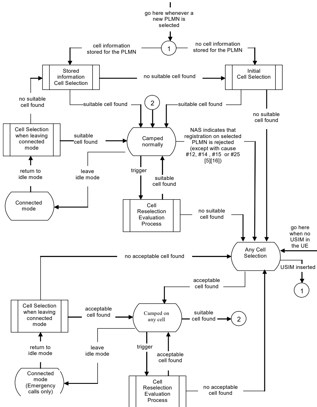
Figure 5.2.2-1: RRC_IDLE Cell Selection and Reselection
