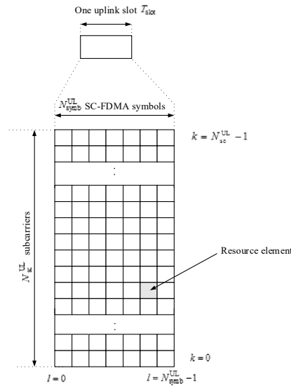
Figure 10.1.2.1-1: Uplink resource grid for NB-IoT
