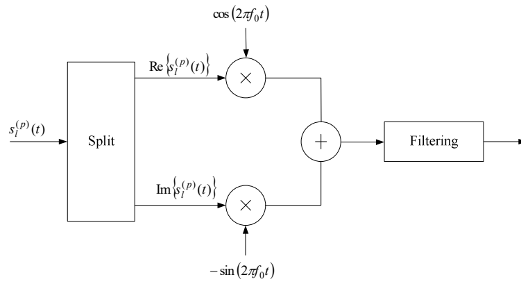
Figure 6.13-1: Downlink modulation
