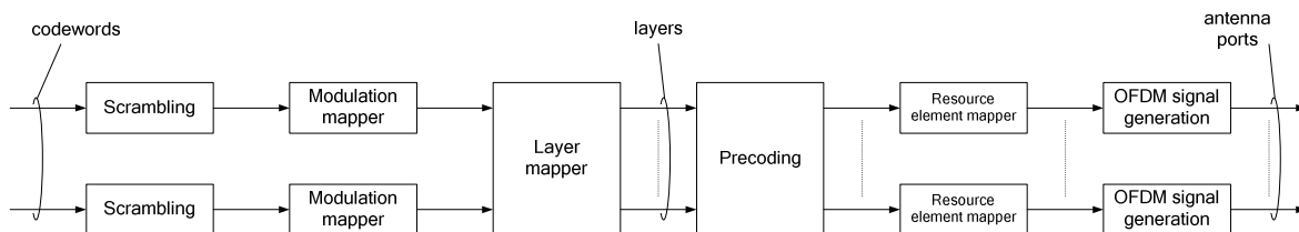
Figure 6.3-1: Overview of physical channel processing
