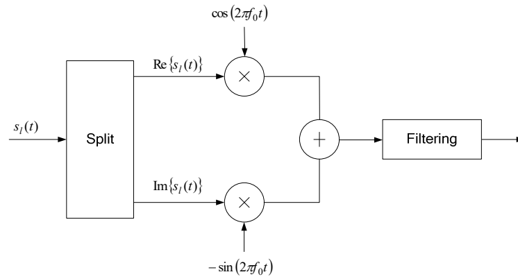
Figure 5.8-1: Uplink modulation
