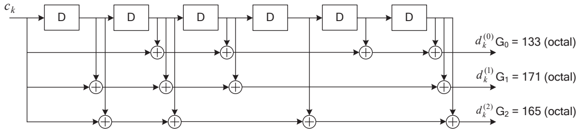
Figure 5.1.3-1: Rate 1/3 tail biting convolutional encoder.
