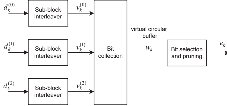
Figure 5.1.4-1. Rate matching for turbo coded transport channels.
