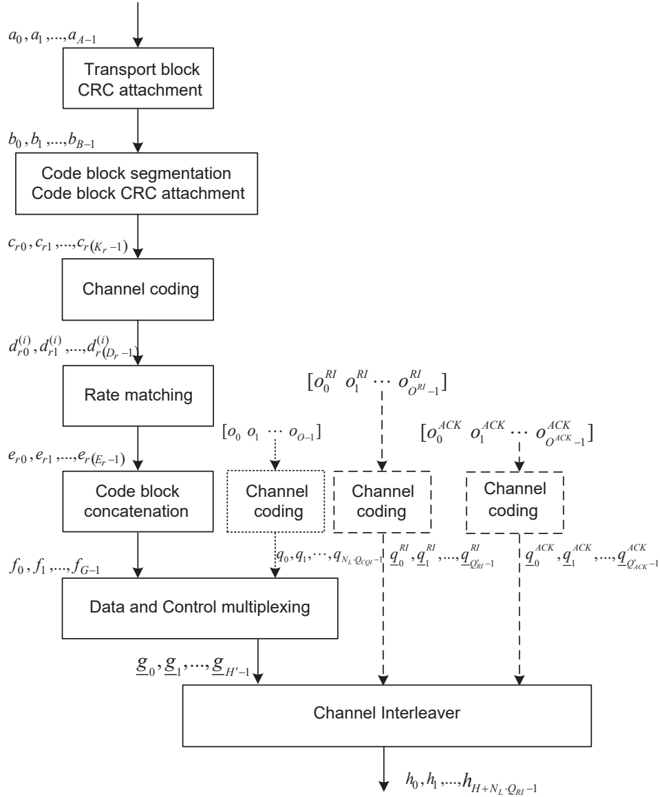
Figure 5.2.2-1: Transport block processing for UL-SCH.
