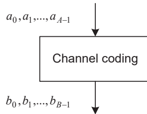
Figure 5.2.3-1: Processing for UCI.
