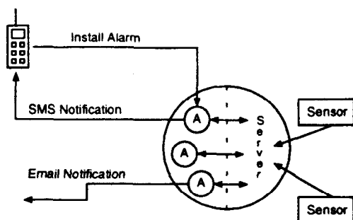
Figure 1: The weather alarm system model. A user client installs an alarm on a remote server. This alarm periodically executes. If the alarm triggers, a notification is sent to the client.
