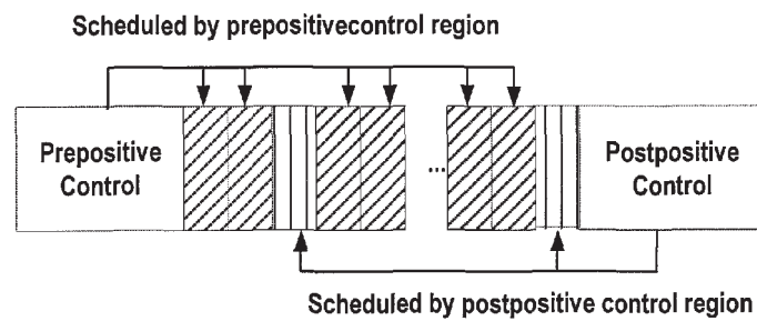
TDM by symbol
