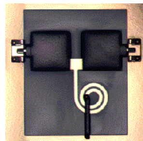
Fig. 2: photograph of an integrated 3 rd -order high pass MCM filter with a size of 1.4mm by 1.7 mm.
