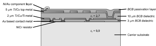
Fig. 1: MCM-D layer architecture developed at IMEC.
