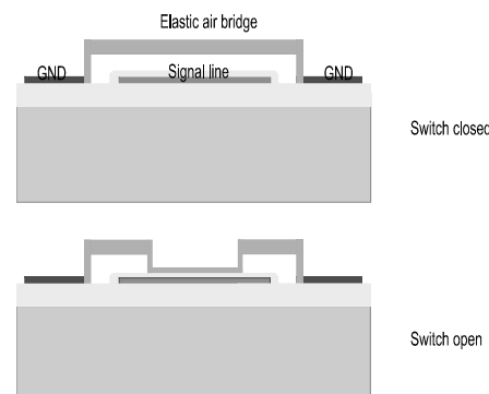
Fig. 3: cross-section of a micromechanical switch.
