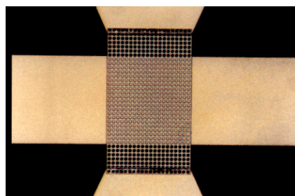
Fig.4: photograph of an RF switch (top view).
