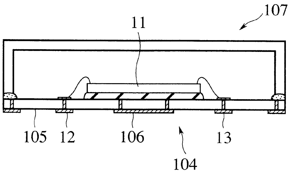
FIG.36B
