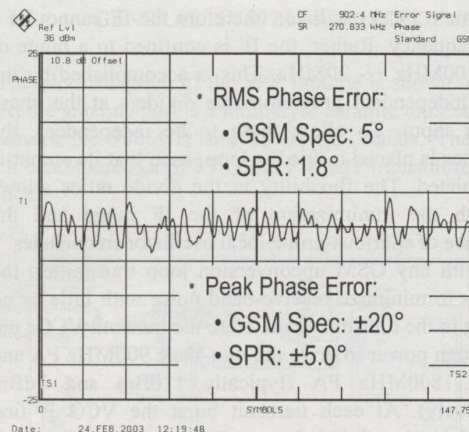
Figure 6 Transmit phase error, EGSM900, 5^\circ/\text{div}
