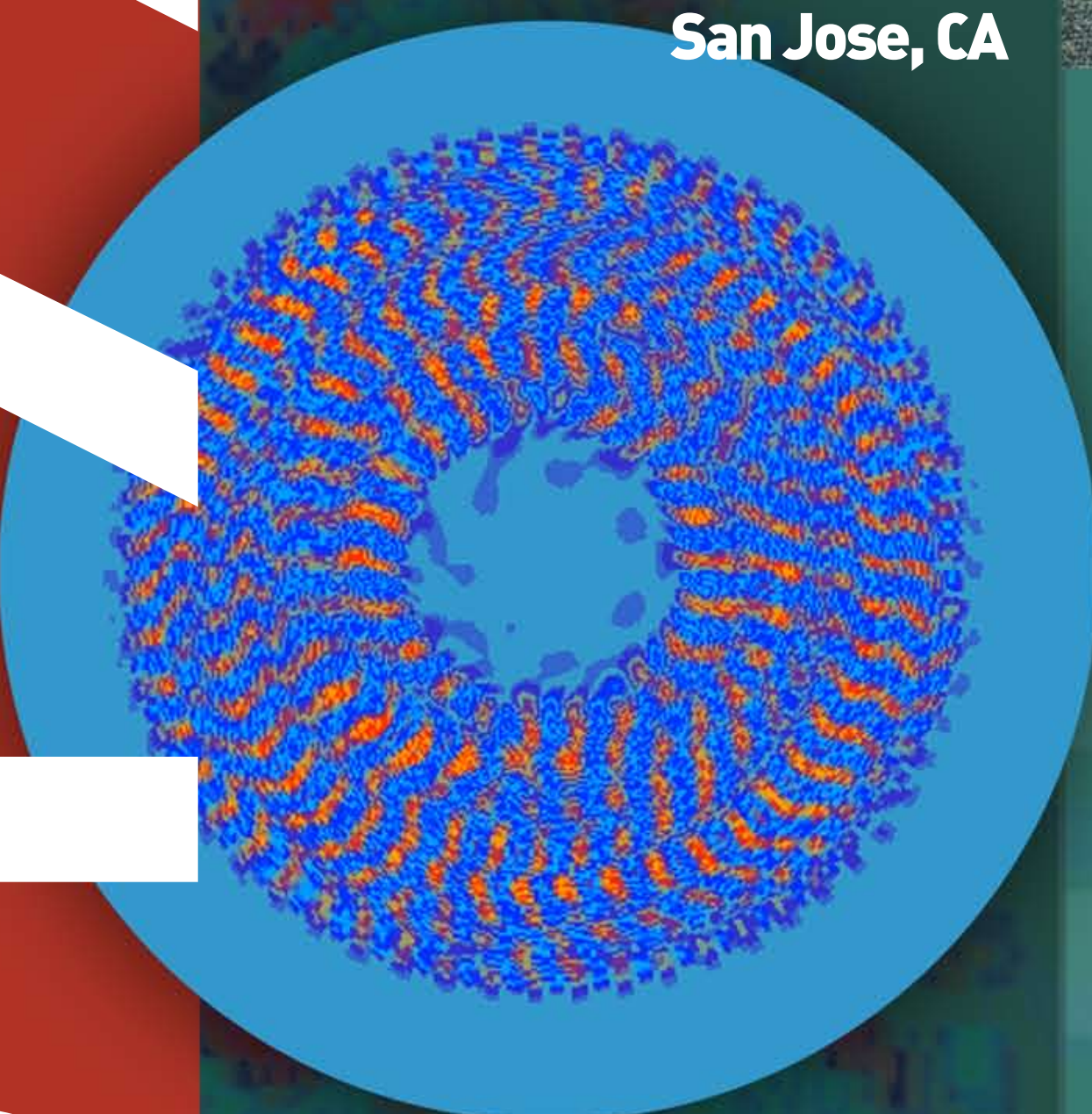
Numerical tokamak model visualization
