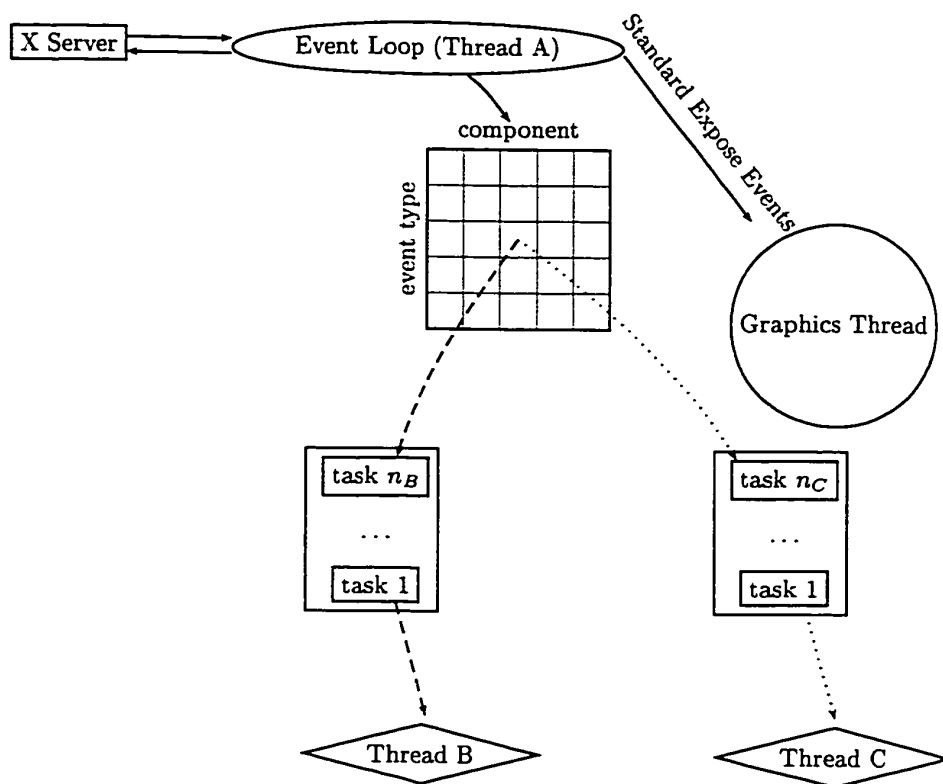
Figure 4.1: GUI Application Control Structure.
