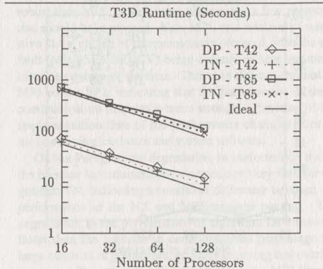
Figure 1. Runtimes for fastest implementations of PSTSWM.
