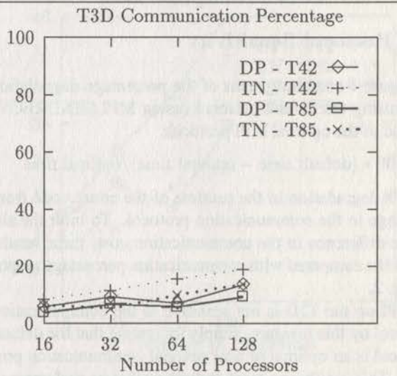
Figure 2. Communication percentages for fastest implementations
