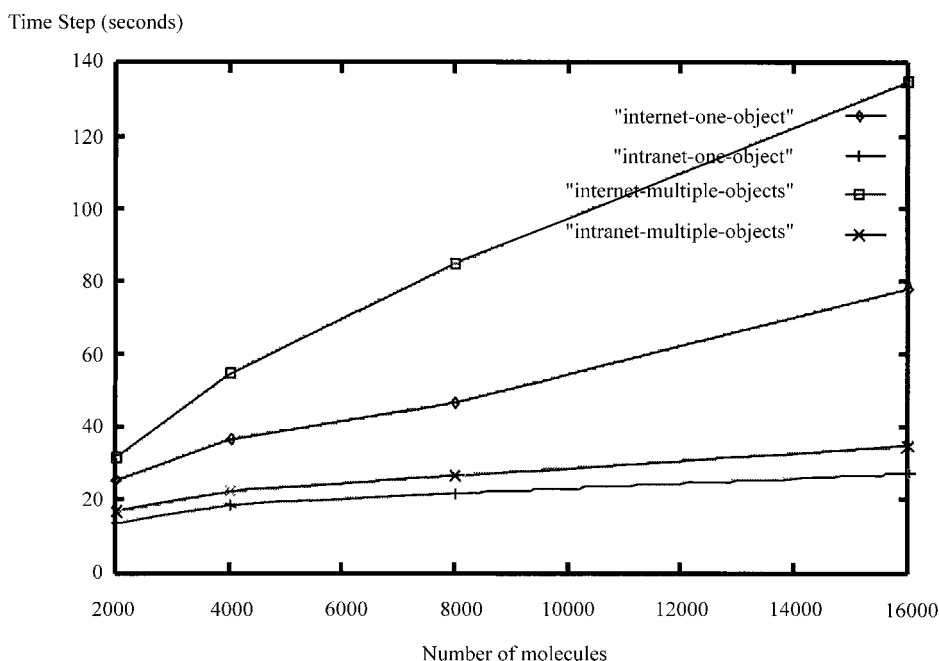
Fig. 5. Performance comparison between wrapping the MD code as a single CORBA object and several different CORBA objects.
