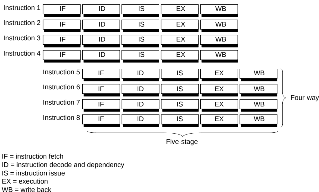
Figure 2-5 Four-Way Superscalar Pipeline
