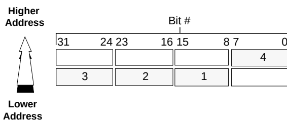
Figure 2-13 Little-Endian Misaligned Word Addressing
