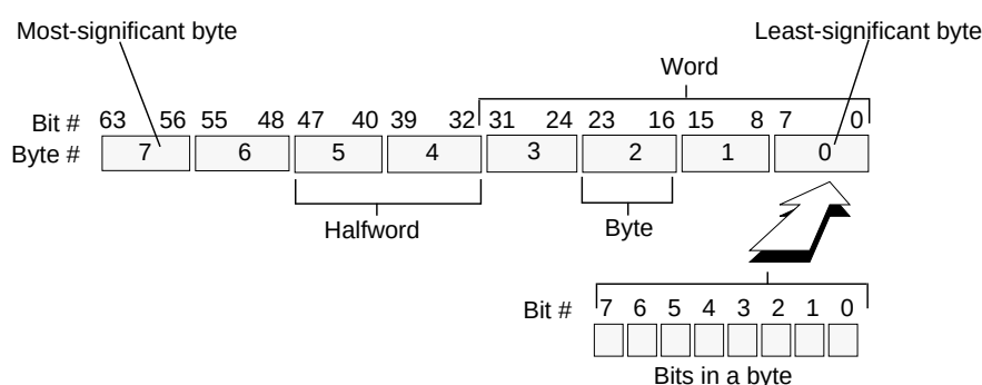
Figure 2-11 Little-Endian Data in Doubleword Format
