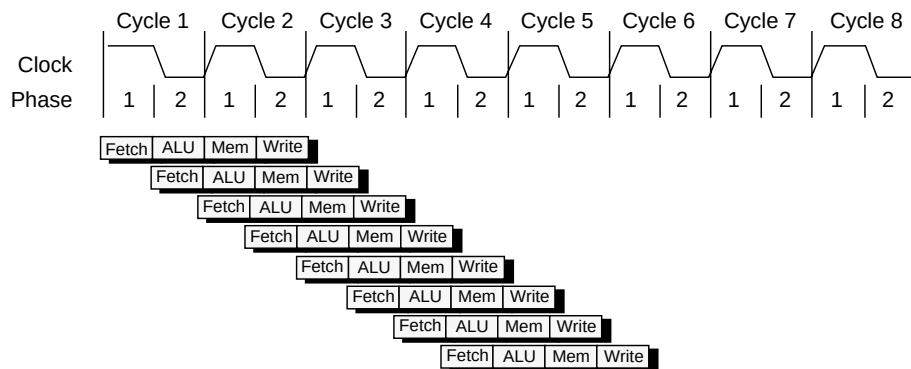
Figure 2-4 Four-Deep Superpipeline
