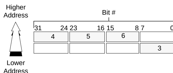
Figure 2-12 Big-Endian Misaligned Word Addressing
