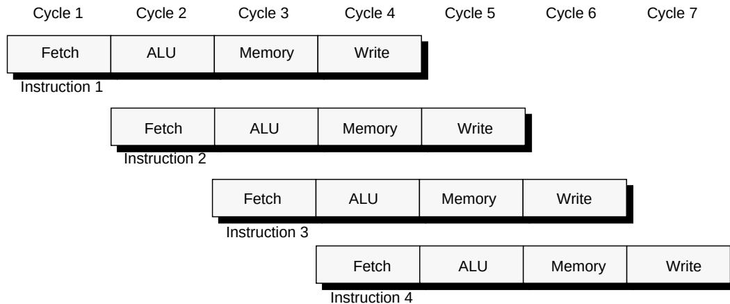
Figure 2-3 Four-Deep Single-Completion Pipeline
