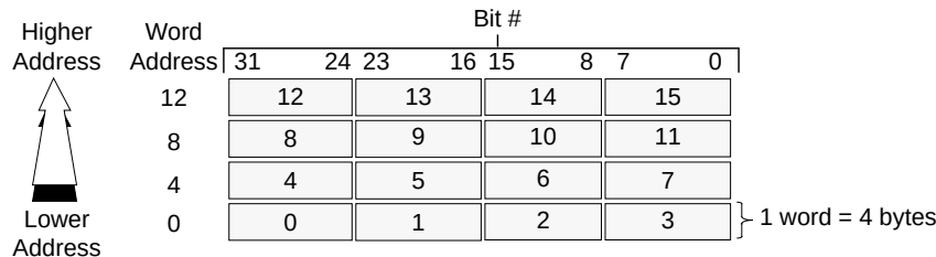
Figure 2-8 Big-Endian Byte Ordering
