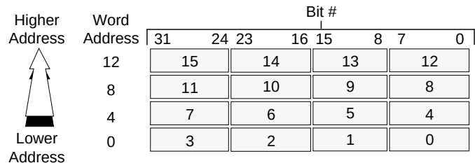
Figure 2-9 Little-Endian Byte Ordering
