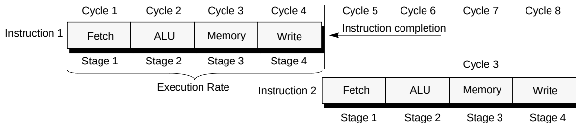
Figure 2-2 One-Deep Single-Completion Instruction Pipeline
