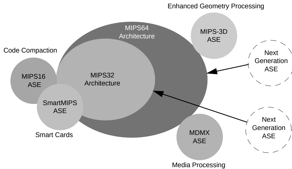
Figure 3-1 MIPS ISAs and ASEs
