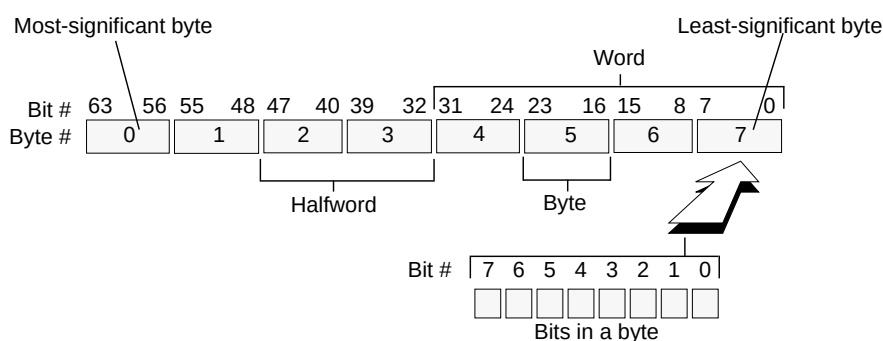
Figure 2-10 Big-Endian Data in Doubleword Format
