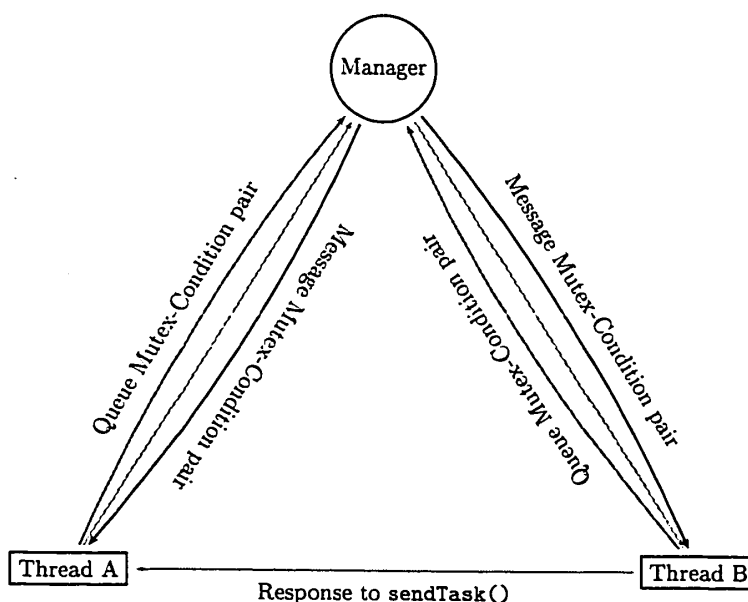
Figure 5.1: Evaluator Manager Communication
