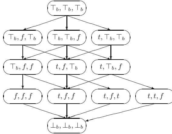
Fig. 2. Visualisation of the type lattice \mathcal{L}_t , of valid triples (\text{real}, \text{logical}, \text{complex}) \in \mathbf{B} \times \mathbf{B} \times \mathbf{B} , where the arrows indicate the partial ordering
